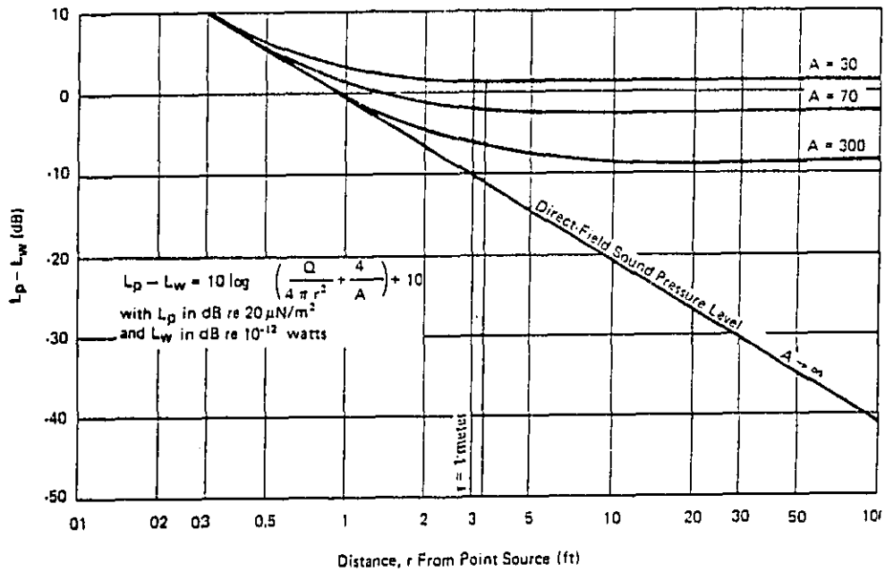
Figure 1-22 Behavior of Sound Indoors, Sound Source Out in Space: (Difference Between Sound Pressure Level and Sound Power Level.)
