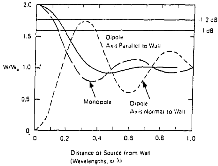
Figure 1-20 Variation in Sound Power Outputs as Source is Moved Away From Reflecting Wall
