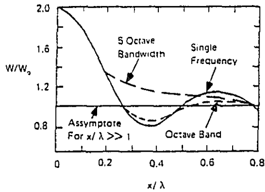
Figure 1-21 Behavior of Sound Source Near a Reflecting Surface. Not much changed by averaging over frequency.
