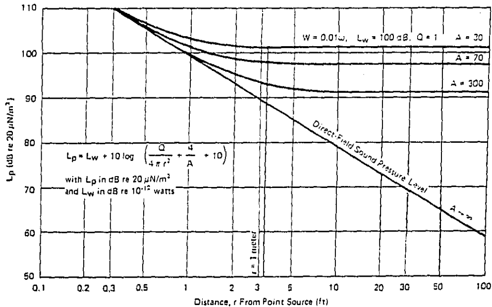
Figure 1-18 Behavior of Sound Indoors, Sound Source Out in Space
