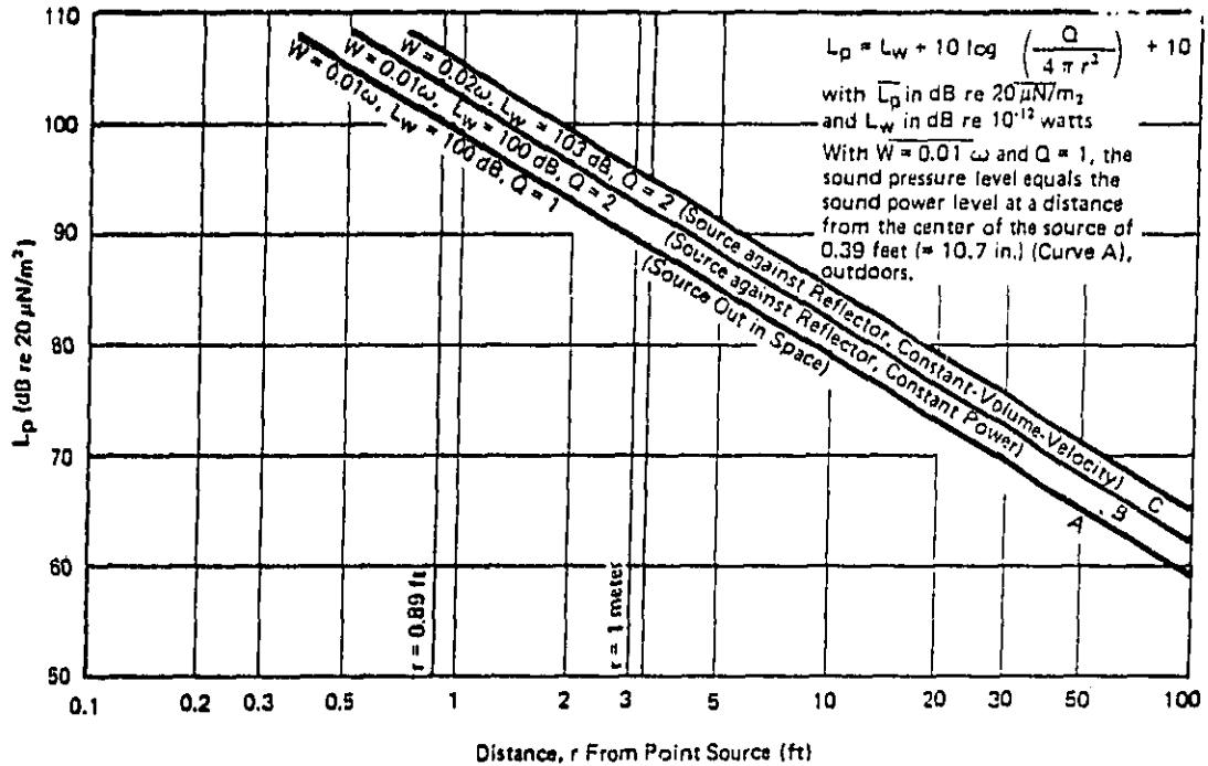
Figure 1-17 Behavior of Sound Outdoors
