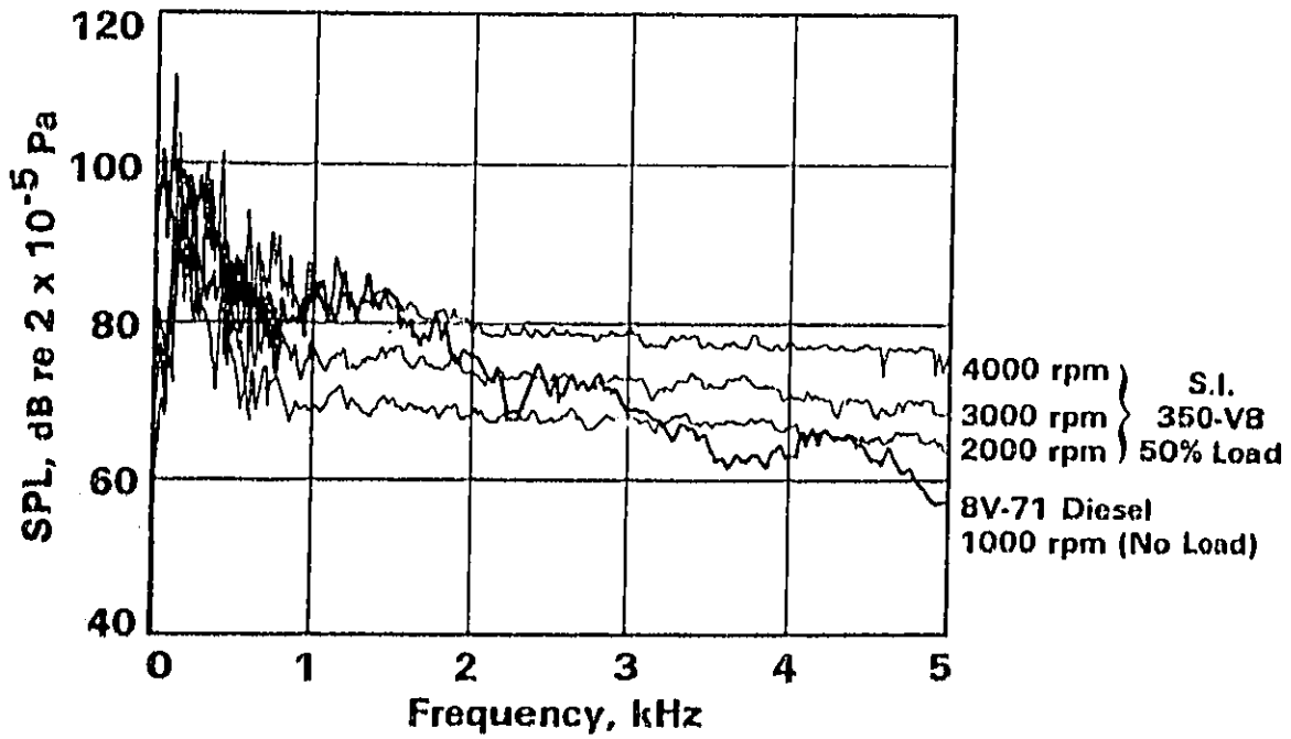
Figure 2. Radiated Exhaust Noise from Two Unsilenced Engines (measured 1.5 m from the end and 45° off the axis of the tailpipe).
