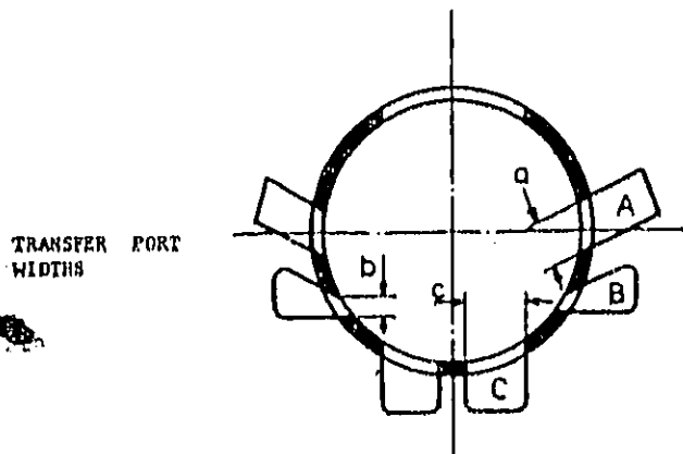
Fig.6 Plan Section through transfer ports
