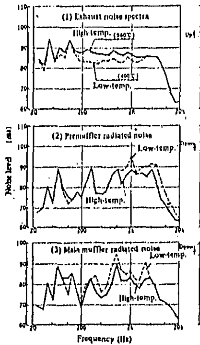
Fig. 21 Influence of exhaust gas temperature on exhaust noise spectra
