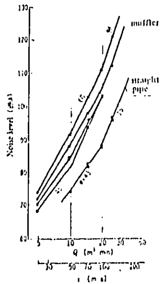
FIG-14 Flow generated noise level under various mufflers
