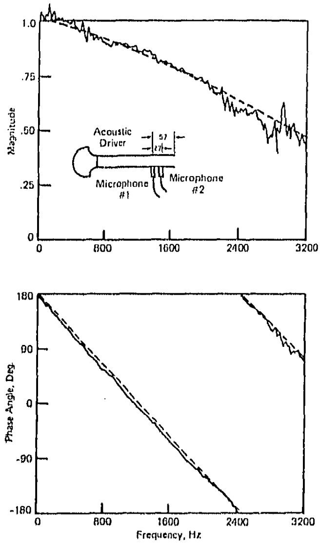
Figure 10. Magnitude and Phase Angle of the Reflection Coefficient for an Open Pipe Termination; --- theory, — experiment, (dimensions in mm).
