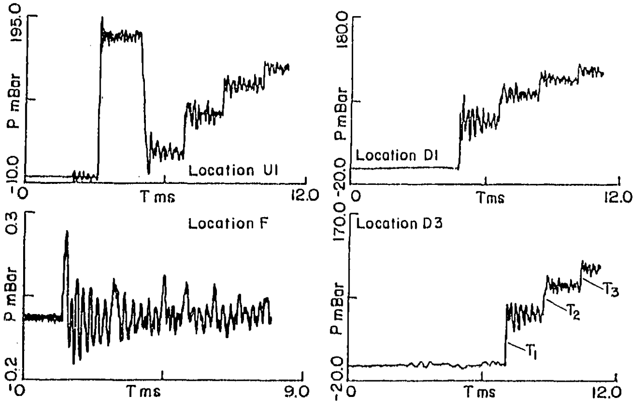
FIGURE 13 PRESSURE HISTORIES OF SHOCK PROPAGATION THROUGH EXPANSION CHAMBER, C. M_s = 1.07 , SHOCK TUBE
