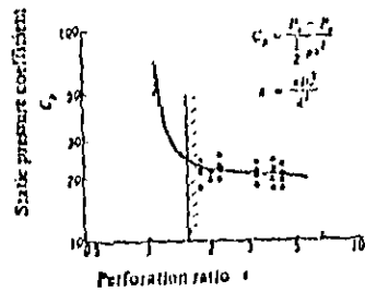
Fig. 14 Static pressure coefficient vs. perforation ratio
