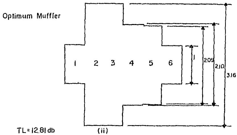
FIG.(5-b) Six Segment Reactive Muffler
