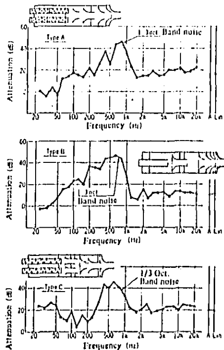
Fig. 5 Attenuation of various test mufflers for vehicles
