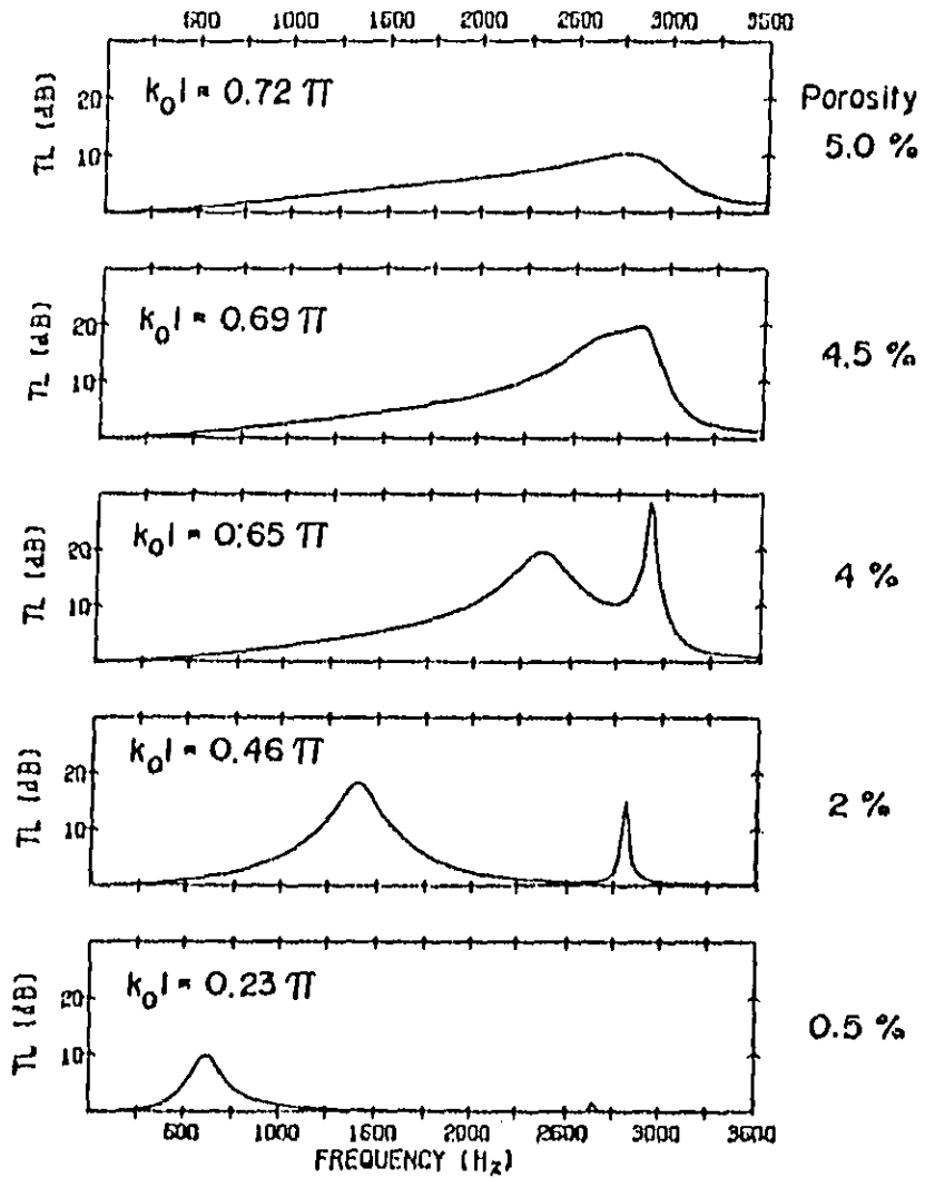
Figure 30. Effect of Porosity on Transmission Loss for a Short Resonator, Predicted From Mathematical Model
