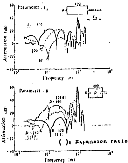
FIG-6 Attenuation of the expansion chamber type mufflers
