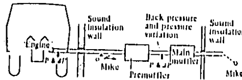
Fig. 19 Experimental layout for the test of exhaust system noise of vehicle
