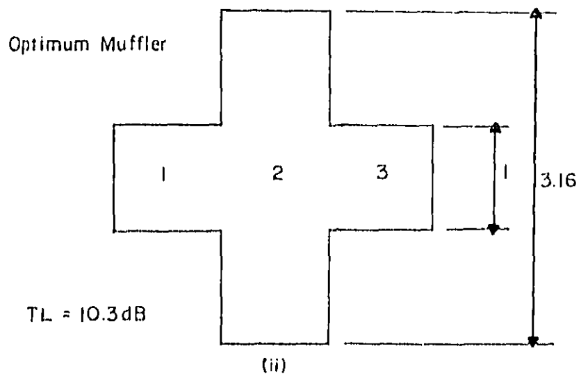
FIG.(4) Three Segment Reactive Muffler
