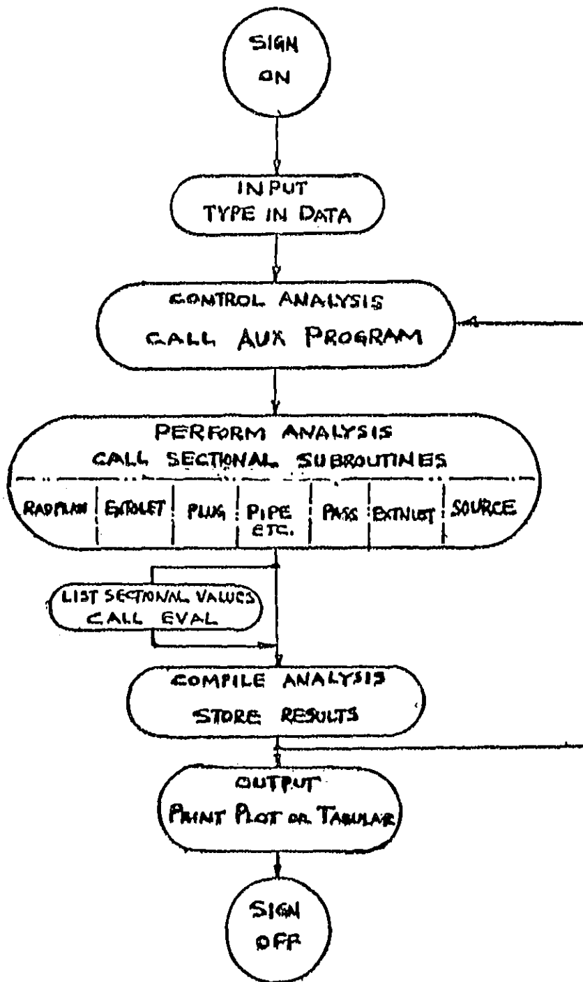
Figure 9. FLOW DIAGRAM FOR SECTIONALIZED MUFFLER DESIGN COMPUTER PROGRAM.
