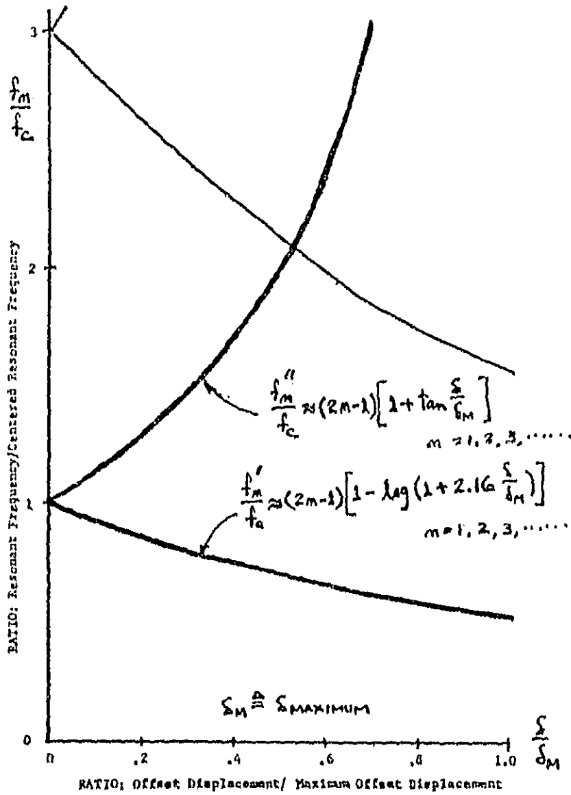
Figure 12. GENERALIZED CURVES FOR RESONANT FREQUENCY VS OFFSET DISPLACEMENT.
