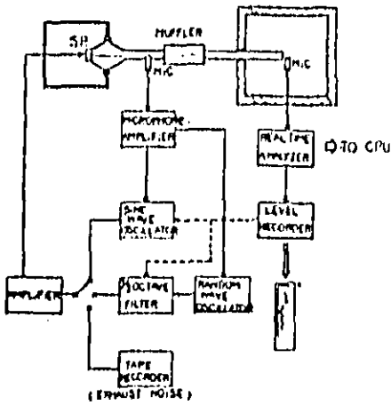
FIG-2 BLOCK DIAGRAM OF ACOUSTIC ATTENUATION MEASURING SYSTEM
