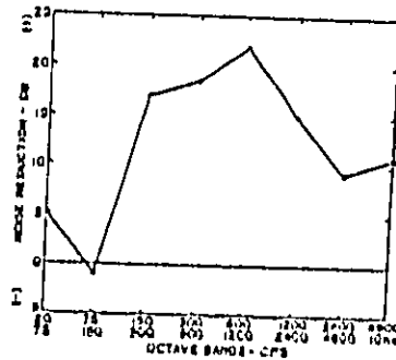
FIGURE 4 Octave Band Analysis of Noise Reduction Figures from Typical Experimental Muffler
