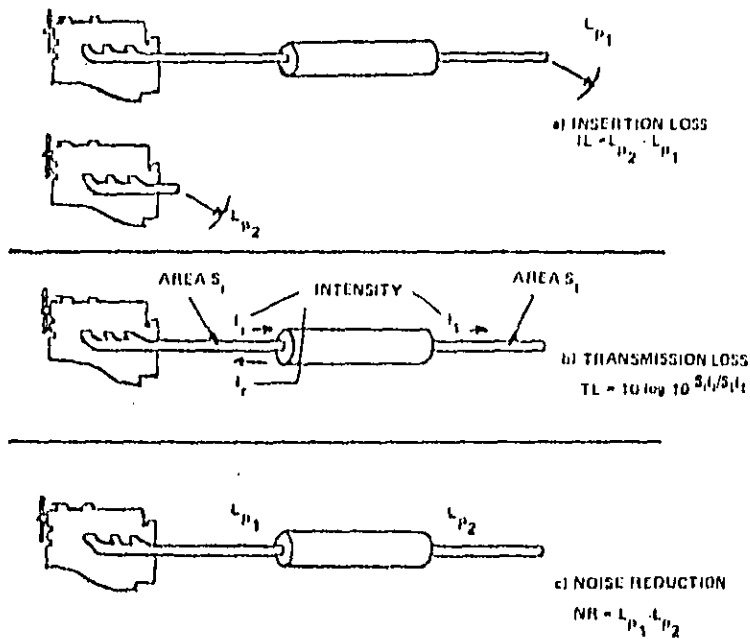
Figure 4. Definitions of Muffler Performance
