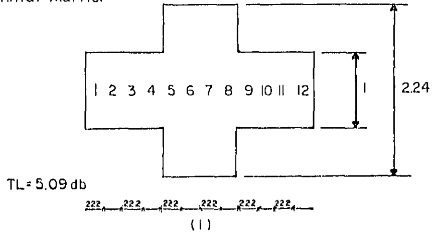
Initial Muffler
