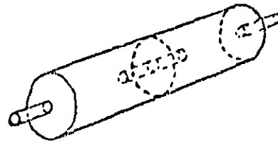
Figure 1b. Double Expansion Chamber With Internal Connecting Tubes
