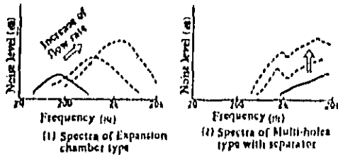
Fig. 10 Change of flow generated noise spectra by air flow rate
