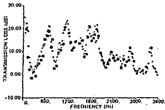
Figure 8. Measured Values of Transmission Loss for Prototype Automotive Muffler. Filled Circle: SWR Method; Open Square, Plus Sign: Two-Microphone Random-Excitation Method
