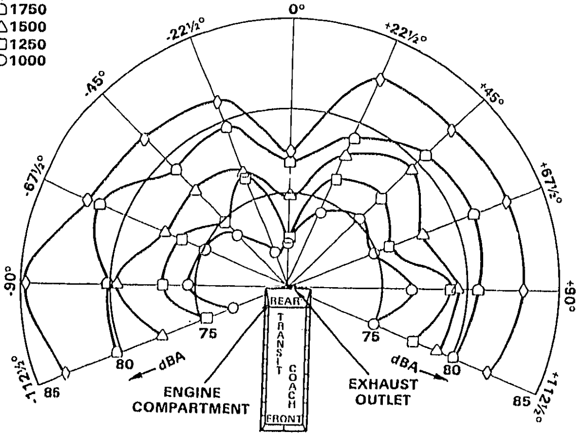
Figure 7. Directivity of Noise from a Transit Coach.
