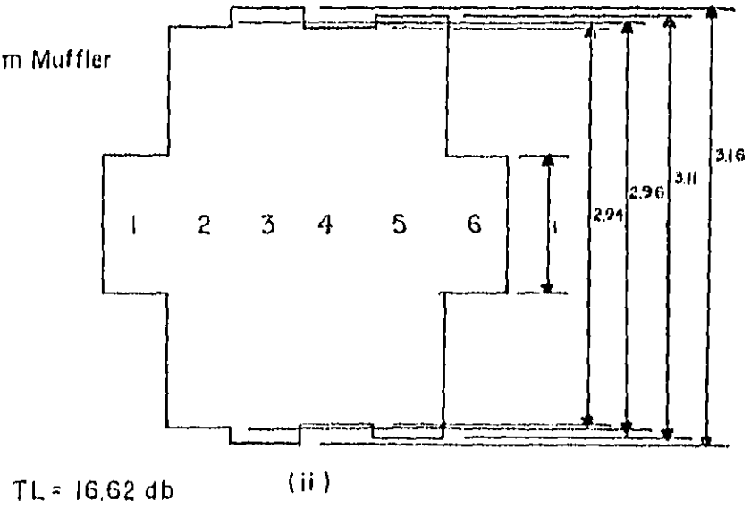
FIG.(5-C) Six Segment Reactive Muffler
