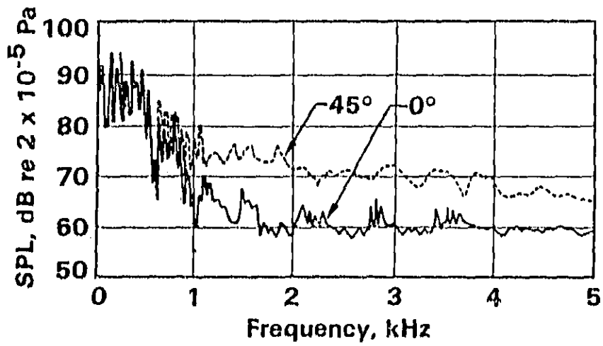
Figure 6. Exhaust Noise Spectra at 0^\circ and 45^\circ from the Tailpipe Axis and 1.5 m from the End of the Tailpipe.
