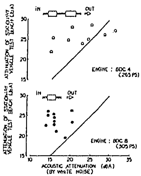
FIG-26 RELATIONSHIP BETWEEN ACOUSTIC ATTENUATION AND ATTENUATION OF STATIONARY VEHICLE
