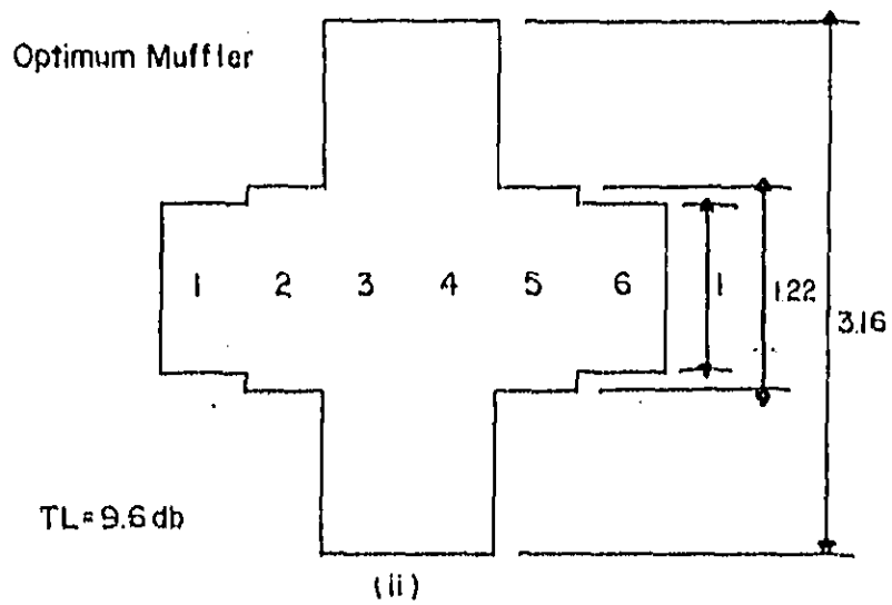
FIG.(5-a) Six Segment Reactive Muffler
