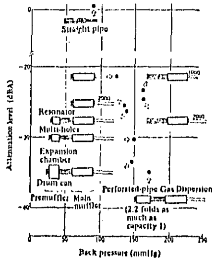
Fig. 22 Relation of exhaust noise reduction and back pressure of various exhaust system arrangements
