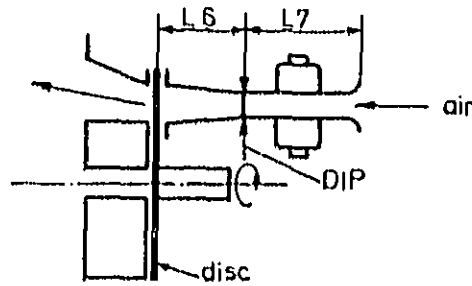
Fig. 9 induction tract length/diameter characteristics for disc valve engines.
