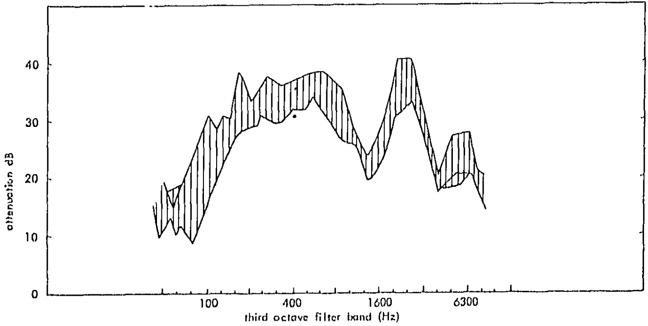
FIG. 16 AVERAGE MEASURED INSERTION LOSS, FULL LOAD TORQUE & SPEEDS, 1000 < N < 2350 rpm. Hatching indicates range of variation.
