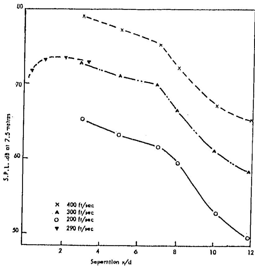
FIG. 6. FLOW NOISE GENERATION IN AXIAL CHAMBERS.
