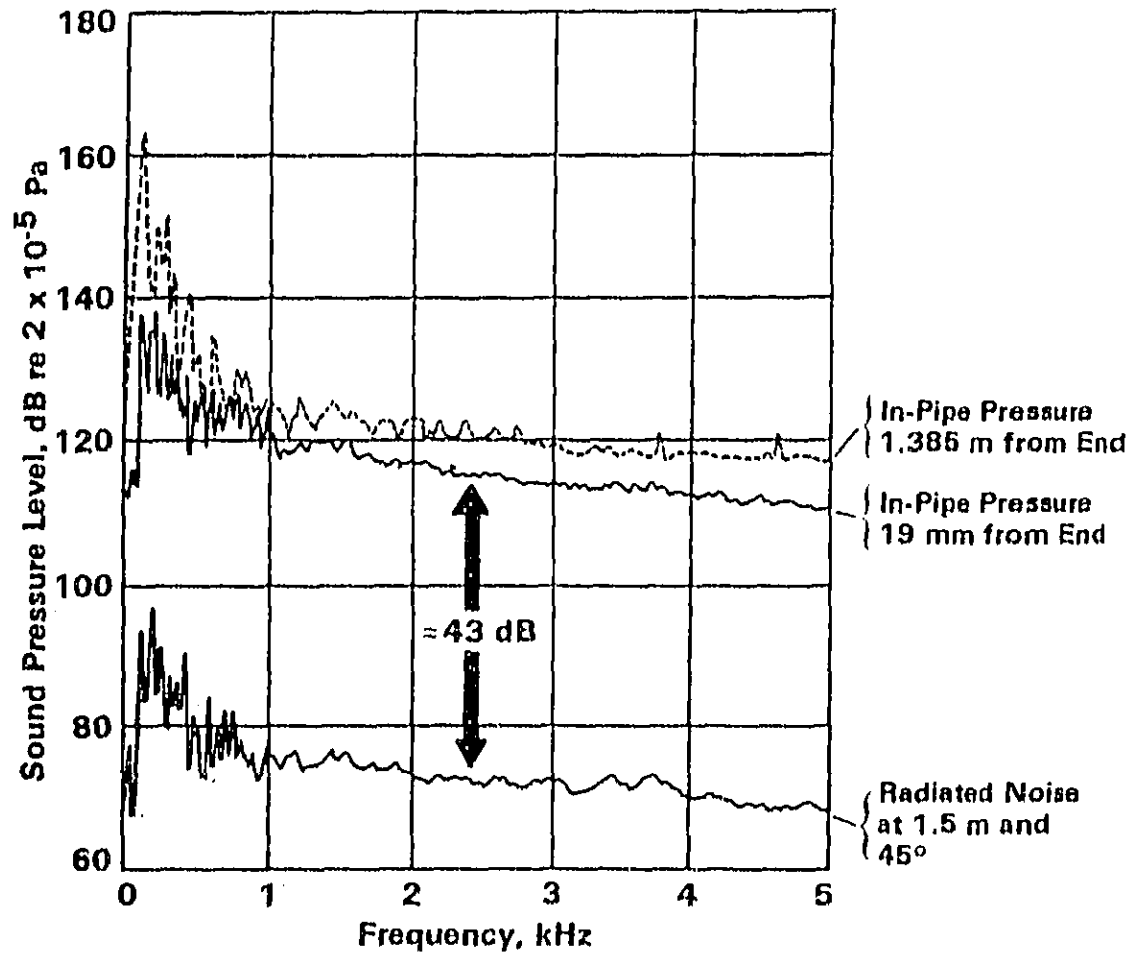
Figure 4. Comparison of Pressure Spectra in the Exhaust Pipe to Radiated Noise Spectra.
