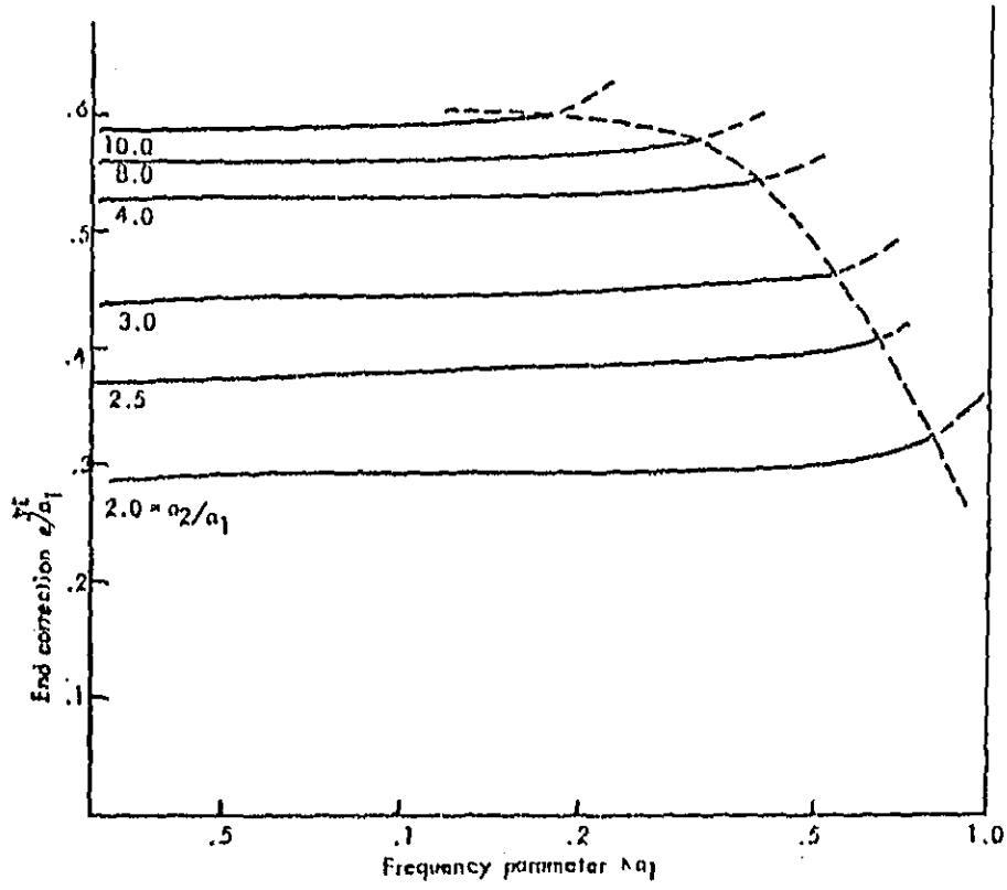
FIG. 3. END CORRECTION FOR EXPANSION OR CONTRACTION.
