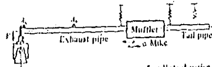
Fig. 15 Testing system of radiated noise from exhaust system
