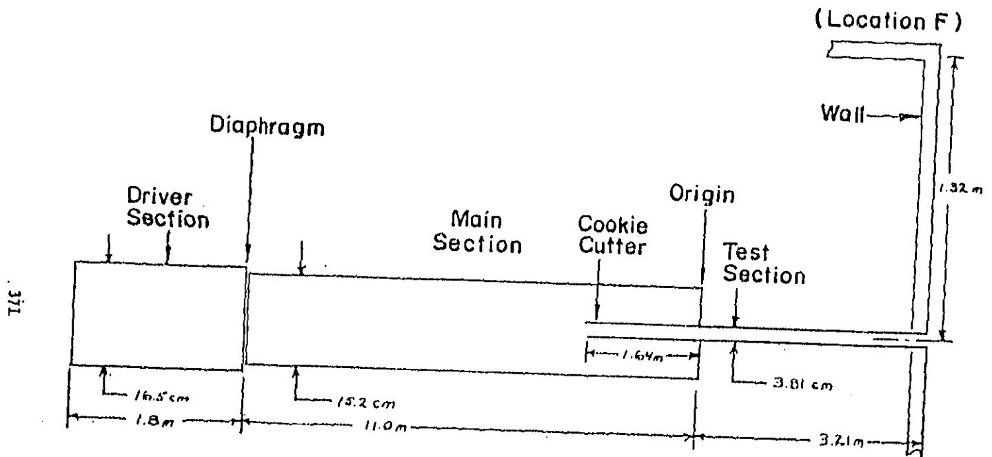
FIGURE 4 GALCIT SIX INCH SHOCK TUBE
