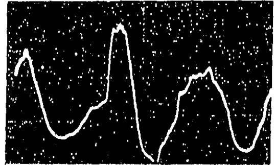
(b) front Vertical scale 138 \frac{mB}{cm} Horizontal scale 1 \frac{mS}{cm}
