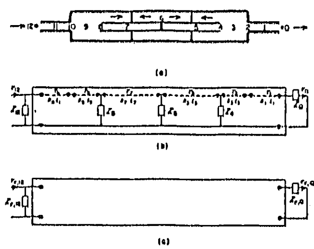
(a) A TYPICAL STRAIGHT-THROUGH EXHAUST MUFFLER (b) ANALOGOUS CIRCUIT FOR THE EVALUATION OF VR_{n+1} (c) ANALOGOUS CIRCUIT FOR THE EVALUATION OF VR_{c,n+1}
