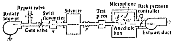
Fig. 6 Experimental layout for flow generated noise
