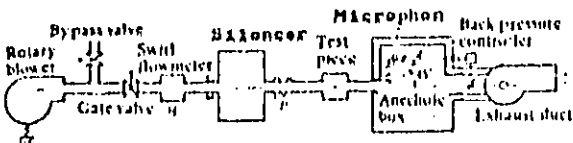
FIG-13 Experimental layout for flow generated noise
