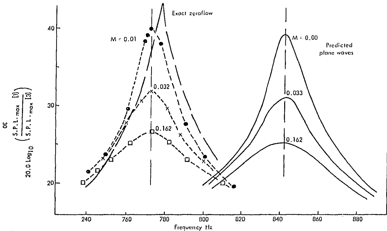
FIG. 1a. ACOUSTIC ENERGY TRANSPORT AT A CONTRACTION WITH SIDEBRANCH.
