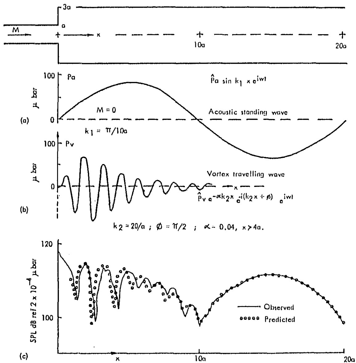
FIG. 11 SOUND PRESSURE LEVEL AFTER A DUCT EXPANSION M = 0.1 ; f = 1250\text{Hz} 2a = 25\text{mm} ; U_c = 0.63 M c_0
