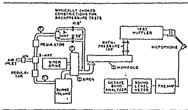
FIGURE 2 Schematic of Bench Test Facility
