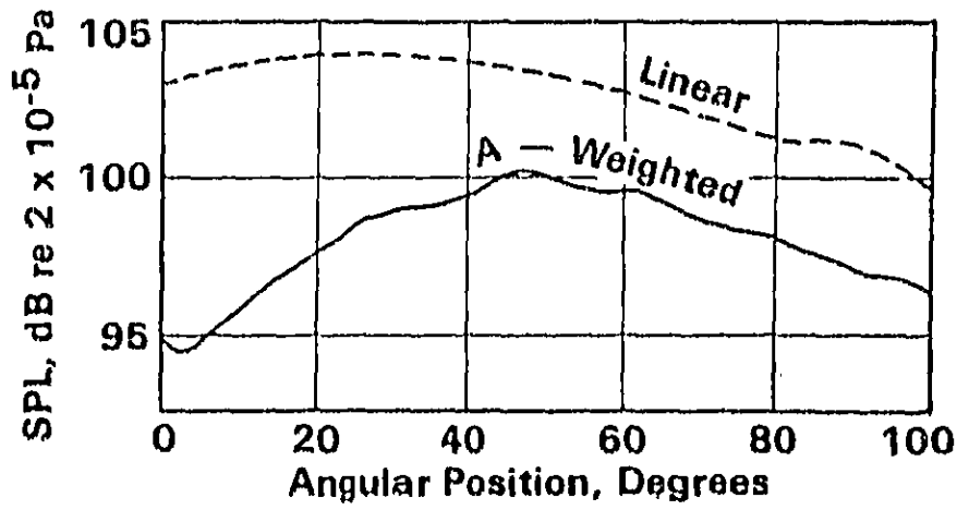
Figure 5. Linear and A-Weighted Exhaust Noise Directivity Measured 1.5 m from the End of the Tailpipe.
