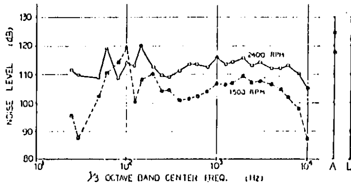
FIG-11 THE SPECTRUM OF EXHAUST NOISE EMITTED FROM ENGINE MANIFOLD
