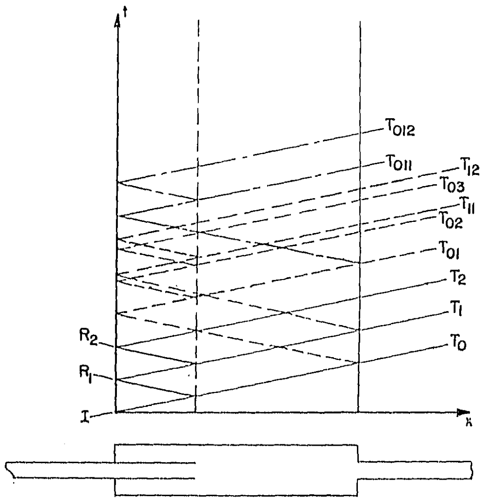
FIGURE 10 EXTENDED INLET SYSTEM
