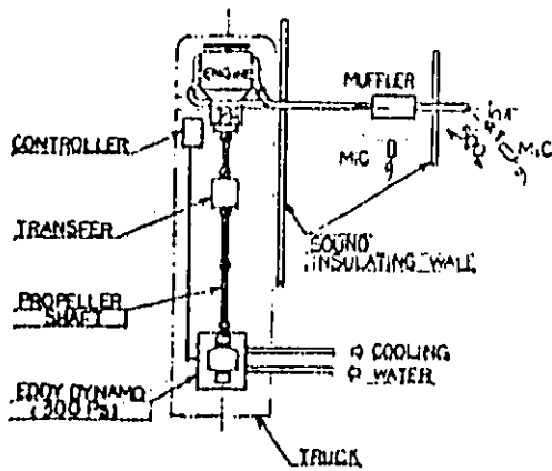
FIG-22 DIAGRAM OF EXHAUST NOISE MEASURING INSTRUMENT ON A STATIONARY VEHICLE
