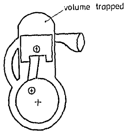
Fig.1 Crankshaft position shown at exhaust closing position, the trapping position, usually EXHOPEN deg BTDC.
