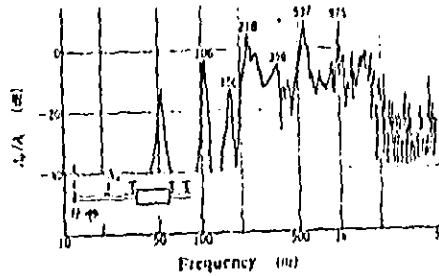
Fig. 16 Vibration response of exhaust system (Random excitation)
