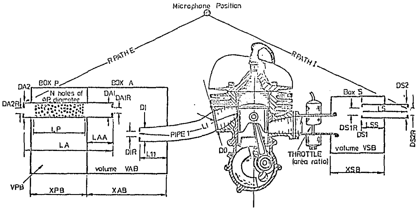
EXHAUST AND INTAKE SILENCING BOX PARAMETERS REQUIRED FOR PROGRAM GPB 5.
