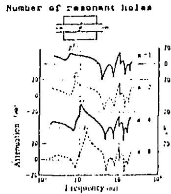
FIG-7 Effect of number of resonant holes
