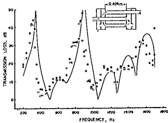
Figure 27. Transmission loss characteristics for combination of C1-SO and S1-SO flow reversing chambers with two resonators; — is predicted; o measured without flow; and e is measured with a flow speed of 32 m/s
