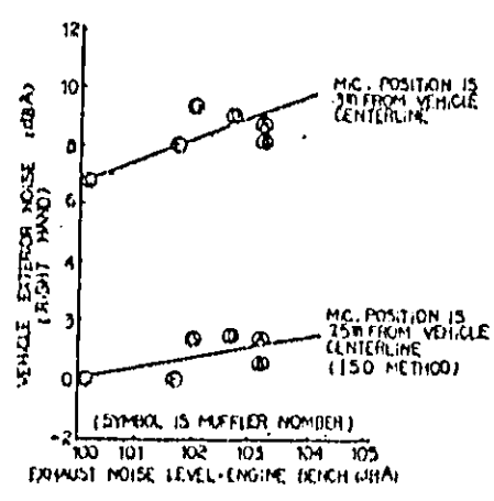
FIG-30. INFLUENCE OF EXHAUST NOISE TO VEHICLE EXTERIOR NOISE
