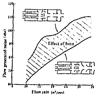
Fig. 12 Reduction of flow generated noise by horn type extension pipe of test muffler for vehicles
