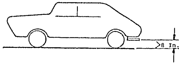
Microphone Height 20" Static Test Layout - Figure 2
