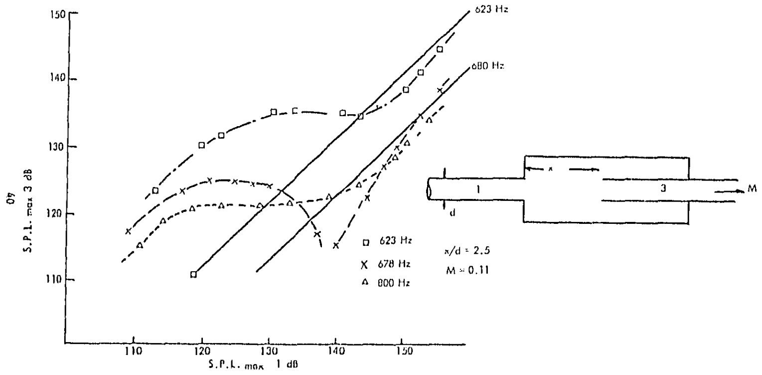
FIG. 9. FLOW ACOUSTIC COUPLING AT AN AREA EXPANSION.
