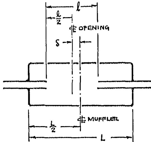
EXTENDED INLET AND OUTLET MUFFLER WITH OFFSET OPENING
