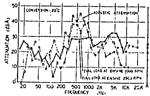
FIG-27 COMPARISON OF ATTENUATION SPECTRUM
