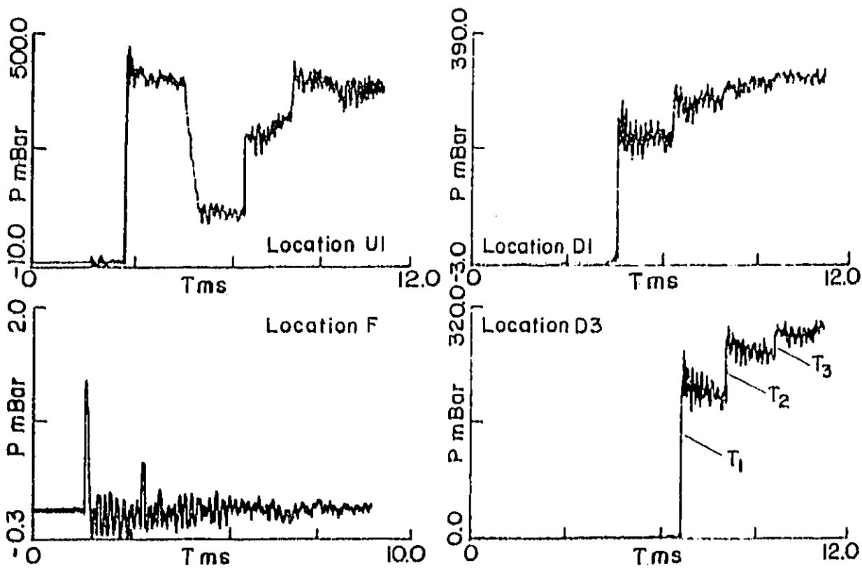
FIGURE 12 PRESSURE HISTORIES OF SHOCK PROPAGATION THROUGH EXPANSION CHAMBER, B. M_s = 1.17 , SHOCK TUBE
