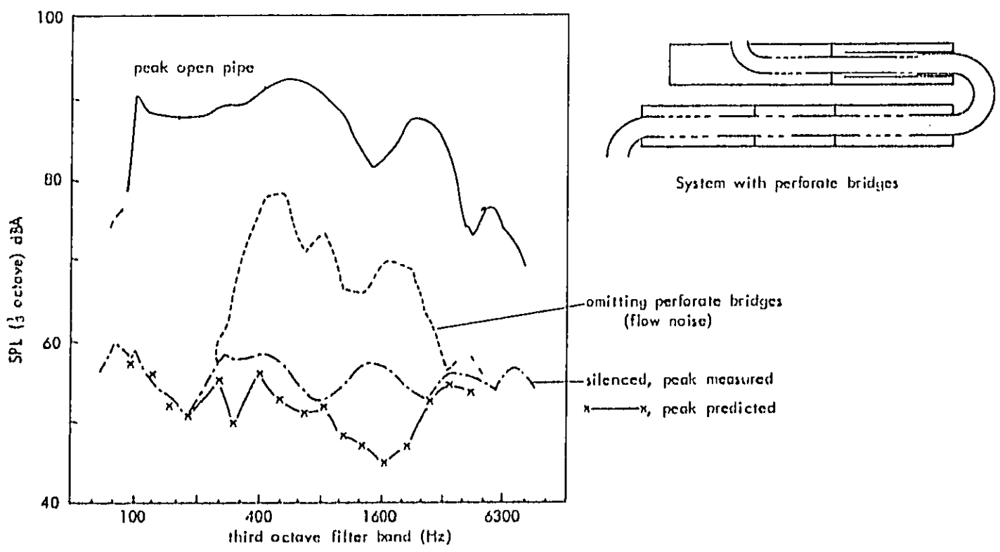
FIG. 15 AVERAGED MEASURED PERFORMANCE. TURBOCHARGED DIESEL AT 7.5m FULL LOAD 8 SPEEDS 1000 < N < 2350
