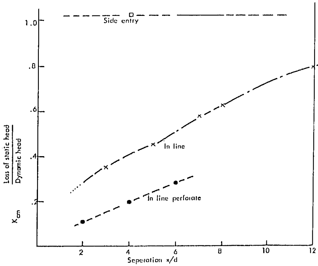
FIG. 8. BACK PRESSURE OF EXPANSION CHAMBERS.
