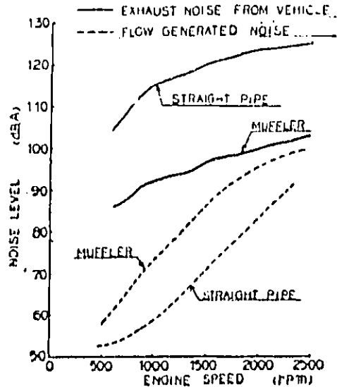
FIG-21 COMPARISON OF EXHAUST NOISE AND FLOW GENERATED NOISE
