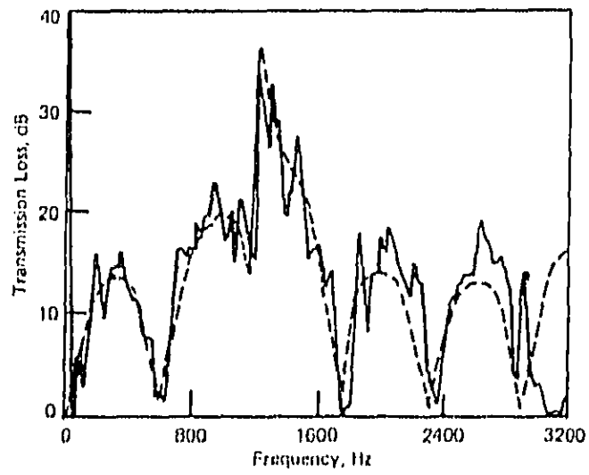
Figure 13. Transmission Loss for the Expansion Chamber Silencer; --- theory, — experiment.
