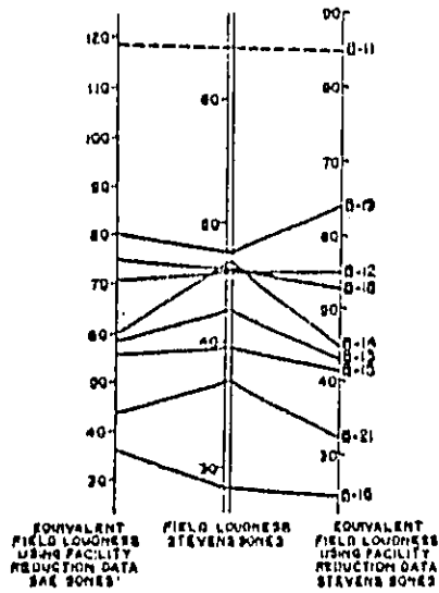
FIGURE 7 Comparison of Field and Facility Evaluations of Muffler Performance
