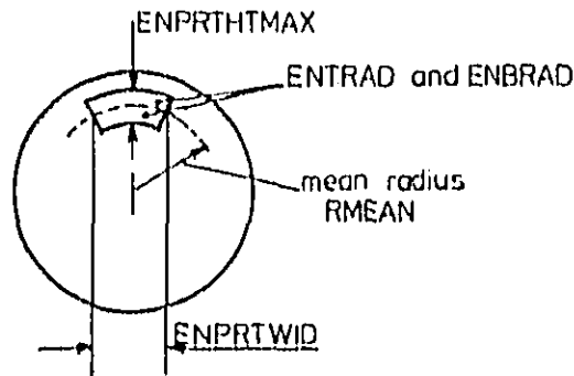
Fig. 8 elevation on face covered by rotary disc
