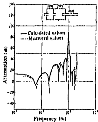
Fig. 2 Comparison of the measured and the calculated muffler attenuations
