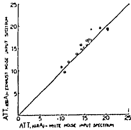
FIG-12 ACOUSTIC ATTENUATION OF MUFFLER
