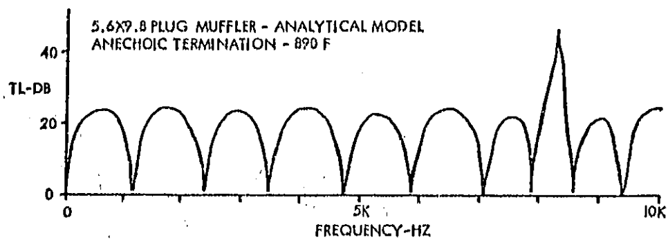
Figure 16. Analytical and Experimental Results for a Plug Muffler.
