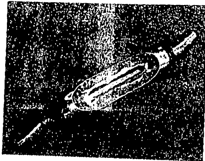
Cutaway View - Glass Pack Muffler Figure 8 426
