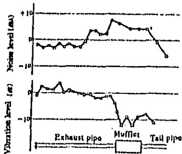
Fig. 23 Example of radiated noise from exhaust system of vehicle
