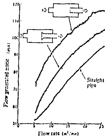
Fig. 11 Reduction of flow generated noise by horn type extension pipe
