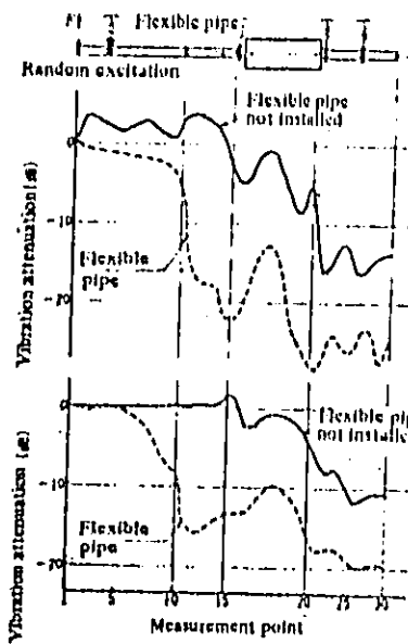
Fig. 18 Reduction of the radiated noise and the vibration of exhaust system by insertion of flexible pipe
