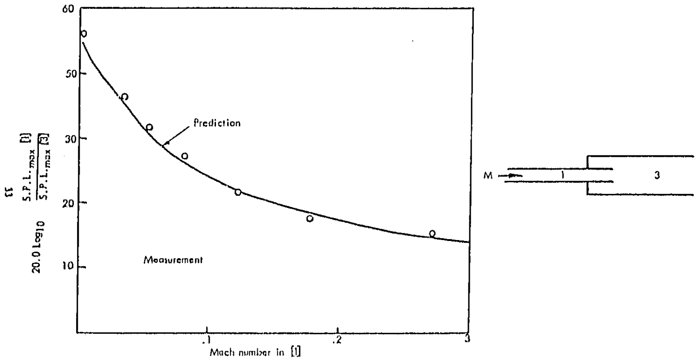
FIG. 2(b). ACOUSTIC ENERGY TRANSPORT AT AN EXPANSION WITH SIDE BRANCH
