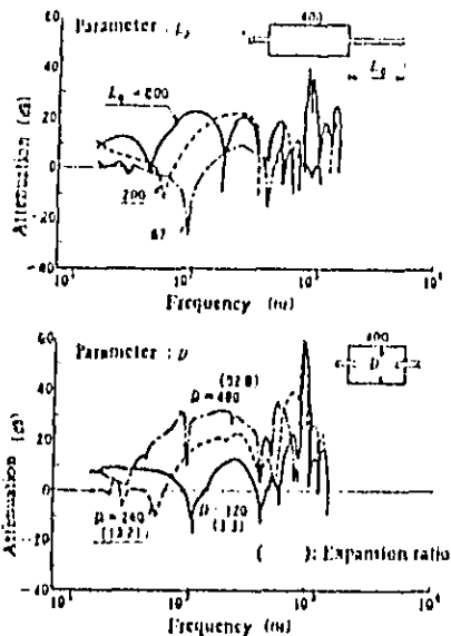
Fig. 3 Attenuation of muffler expansion chamber type
