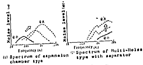
FIG-16 Change of flow generated noise spectra by air flow rate
