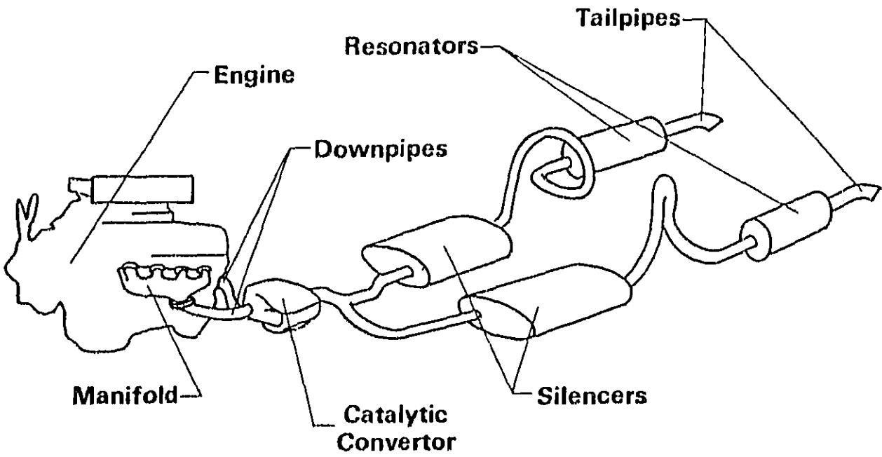
Figure 1. Components of an Engine Exhaust System.
