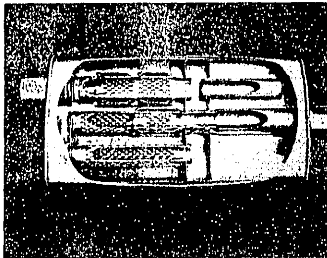
Cutaway View - Regular Aftermarket Muffler Figure 4
