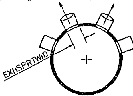
Fig.3 Plan section on exhaust ports
