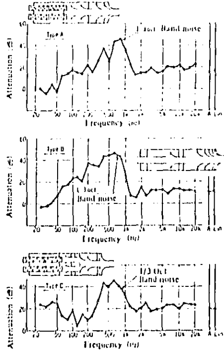
FIG-9 Acoustic attenuation of various test mufflers
