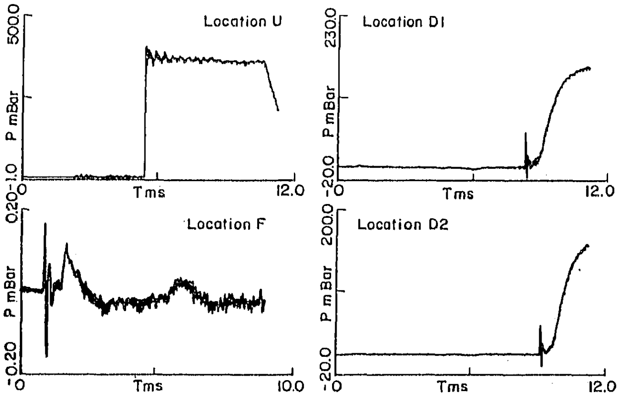
FIGURE 7 PRESSURE HISTORIES OF SHOCK PROPAGATION PAST A PERFORATED TUBE A_E/A = 4.00 , SHOCK TUBE
