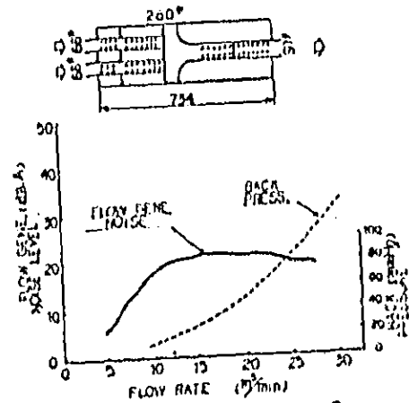
FIG-18 EXAMPLE OF FLOW GENERATED NOISE
