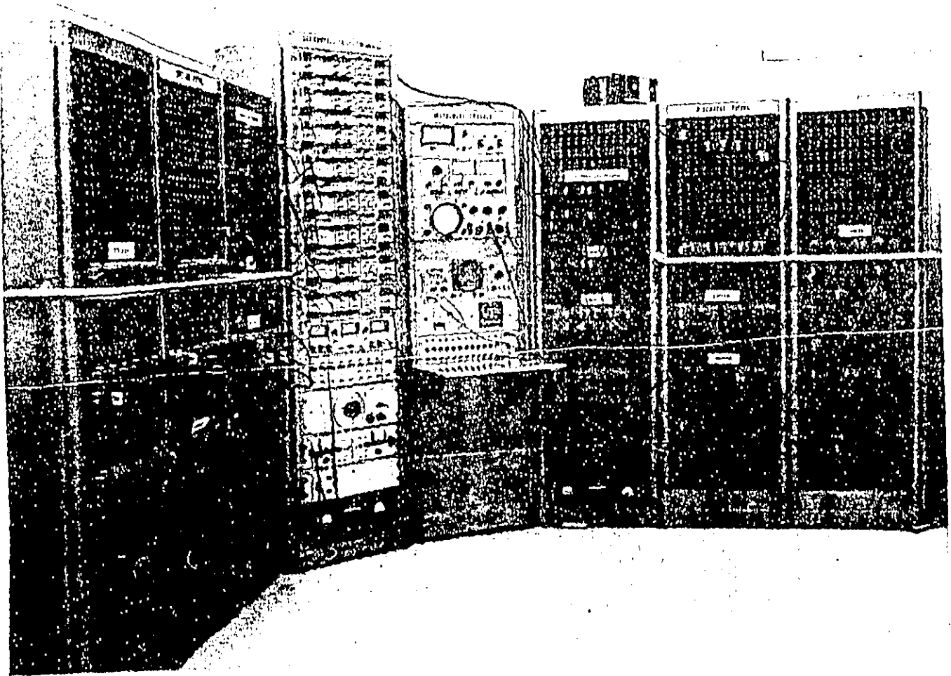
FIGURE 10 Electroacoustic Analog for Simulation of the Acoustic Response of Piping Systems
