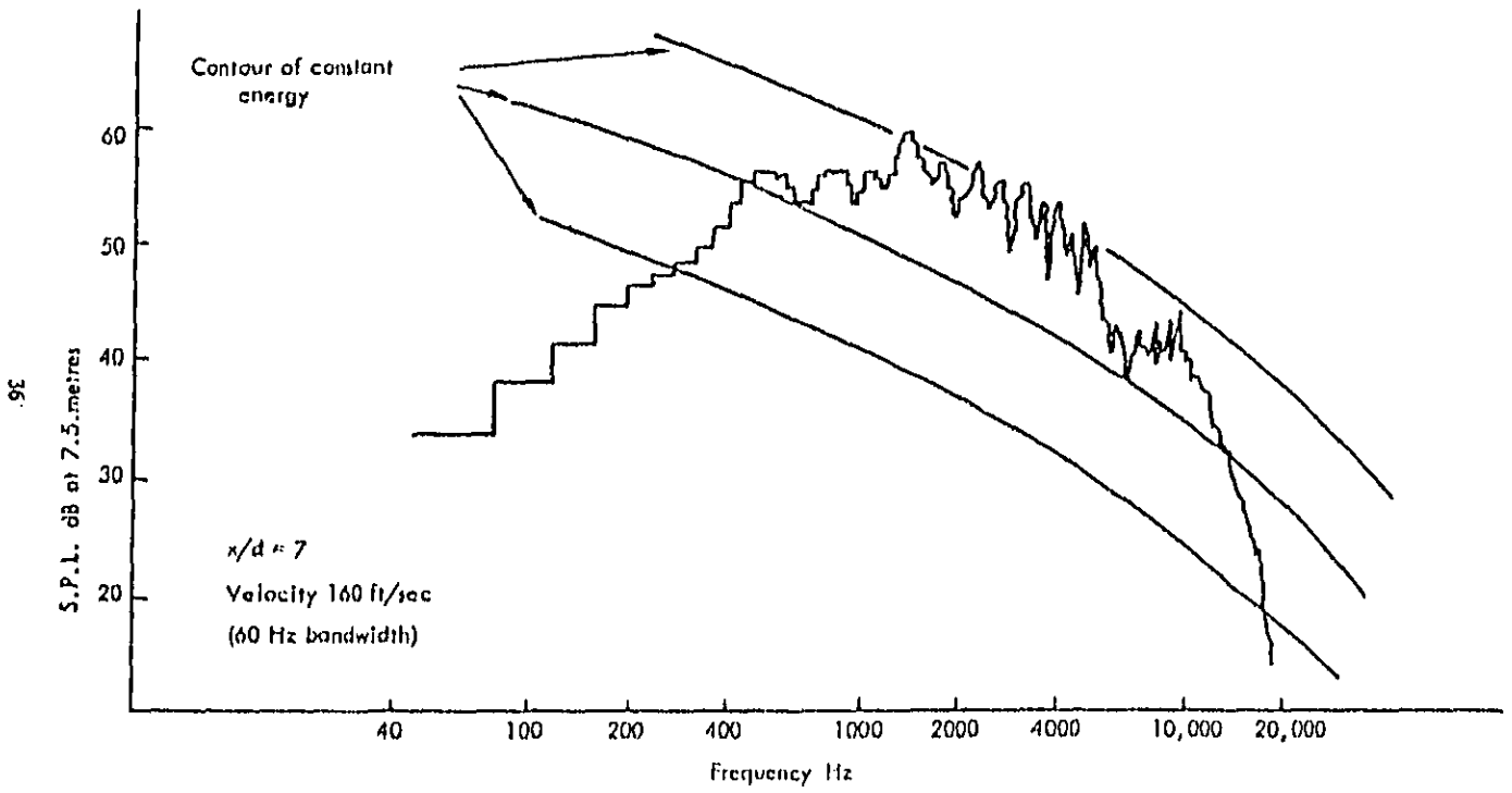
FIG. 5. SPECTRAL CONTENT OF FLOW NOISE
