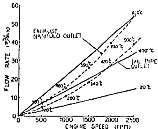
FIG-20 RELATION BETWEEN ENGINE SPEED AND EXHAUST GAS FLOW
