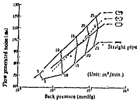
Fig. 9 Flow generated noise of expansion type mufflers
