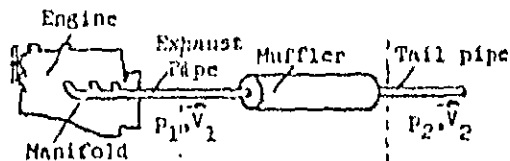
Figure 13a. Real Engine-Muffler-Exhaust System
