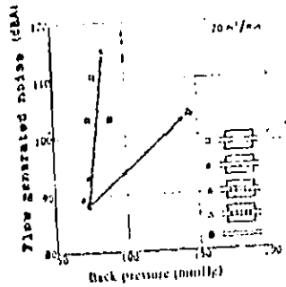
FIG-15 Relation of flow generated noise and back pressure of typical muffler elements
