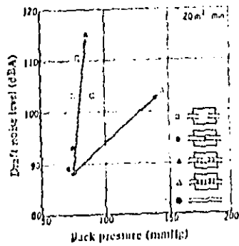
Fig. 13 Relation of flow generated noise and back pressure of typical muffler elements
