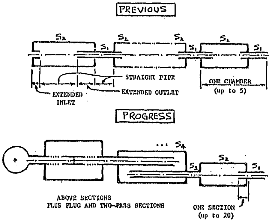
Figure 7. EXTENSIONS TO NASA MUFFLER DESIGN COMPUTER PROGRAM.
