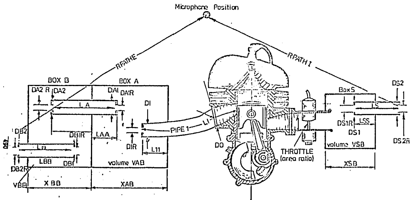
Program: G.P.B. 3 EXHAUST AND INTAKE SILENCING BOX PARAMETERS REQUIRED FOR PROGRAM
