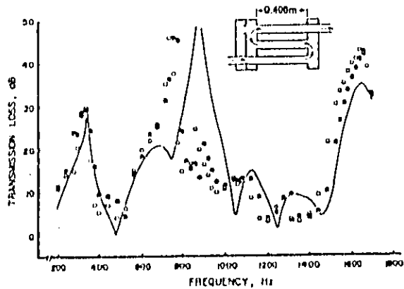
Figure 26. Transmission loss characteristics for combination of S1-CO and C1-SO flow reversing chambers; — is predicted; o is measured without flow and e is measured with a flow speed of 32 m/s
