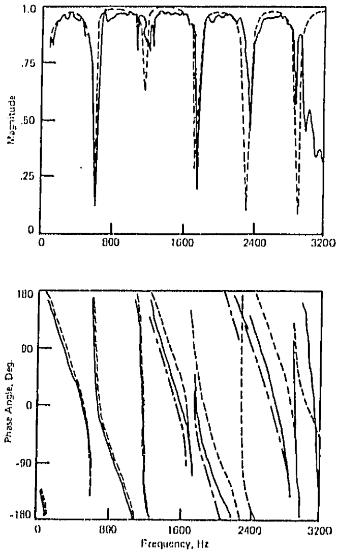
Figure 12. Magnitude and Phase Angle of the Reflection Coefficient for the Expansion Chamber Silencer; --- theory, - - - modified theory, — experiment.
