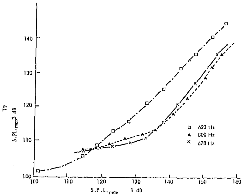
FIG. 10. SUPPRESSION OF FLOW-ACOUSTIC COUPLING BY A BRIDGE PERFORATE.
