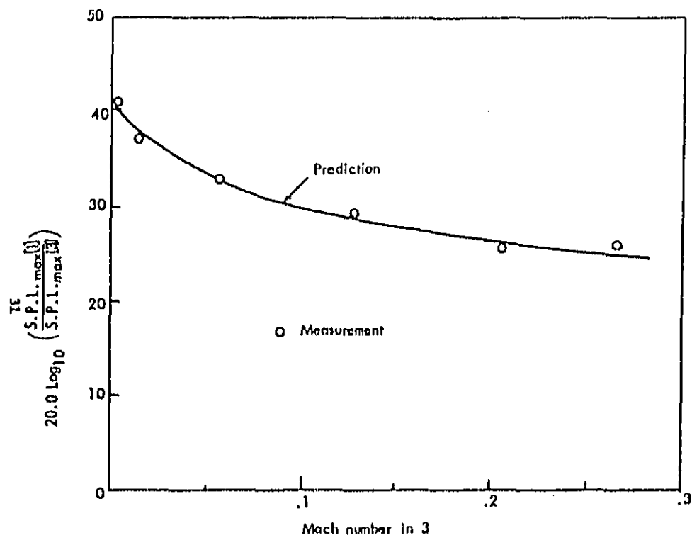
FIG. 1(b) ACOUSTIC ENERGY TRANSPORT AT A CONTRACTION WITH SIDEBRANCH.
