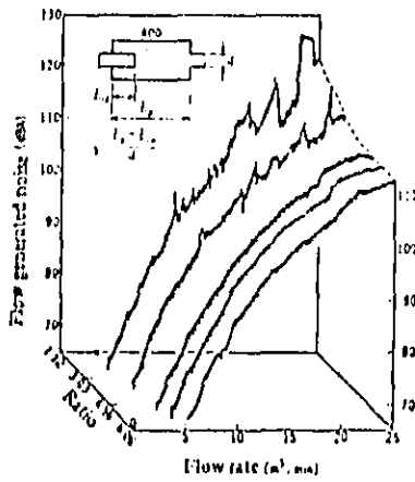
Fig. 8 Effect of the gap of inlet and outlet expansion pipe to flow generated noise
