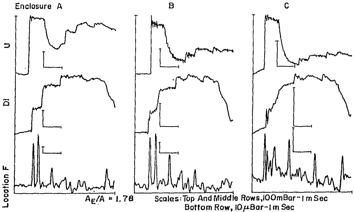
FIGURE 8 PRESSURE HISTORIES OF SHOCK PROPAGATION PAST PERFORATED TUBES, RESONANCE TUBE
