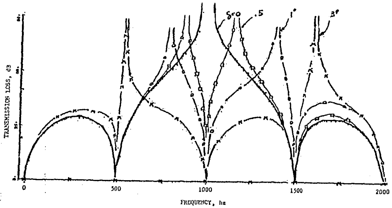
Figure 11. FAMILY OF TRANSMISSION LOSS CURVES FOR SEVERAL AMOUNTS OF OFFSET PIPE OPENING.
