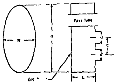
Figure 19. Flow-Reversing Chamber With Pass Tube and End Plate. C - Distance Between Centers of Inlet and Outlet Tubes; H - Height of Chamber; L - Length of Chamber; W - Width of Chamber; and d - pipe Diameter
