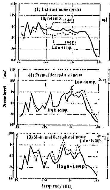
FIG-24 Influence of exhaust gas temperature on exhaust noise spectra
