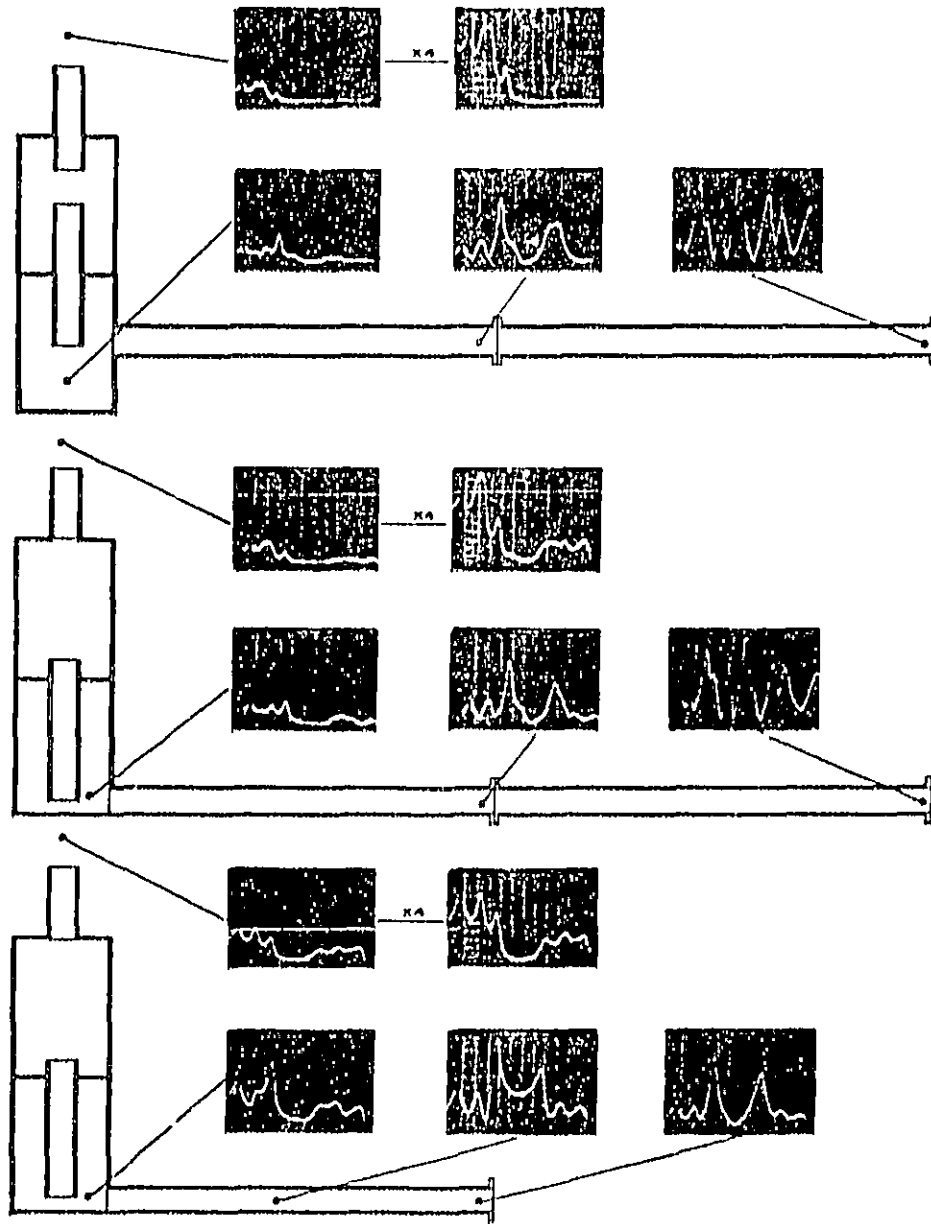
Huffler and Exhaust System Performance Characteristics as Recorded on the Electroacoustic Analog FIGURE 13
