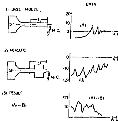
FIG-3 ACOUSTIC ATTENUATION
