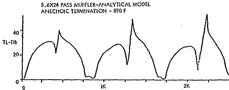
Figure 15. Analytical and Experimental Results for a Pass Muffler.
