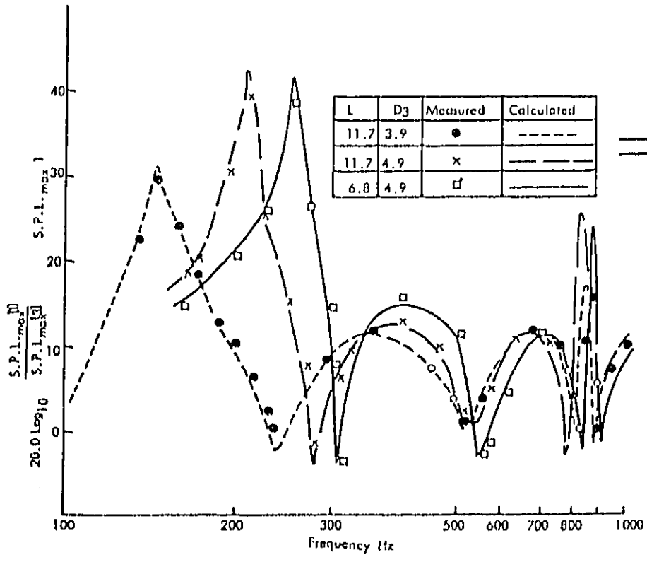
FIG. 4. PERFORMANCE OF FOLDED CHAMBERS.
