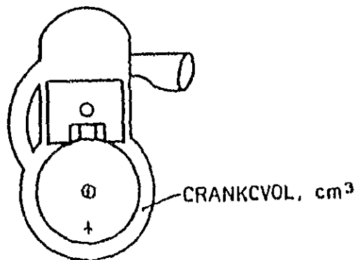
Fig.2 Crankshaft position shown at bottom dead centre, B.D.C. - note all transfer ducts are open, and the volume under the piston is then the crankcase clearance volume, measured in \text{cm}^3 . If SV is the swept volume per cylinder, \text{cm}^3 then -
