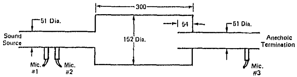
Figure 11. Expansion Chamber Silencer (dimensions in mm).
