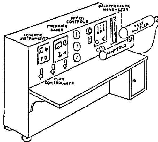
FIGURE 9 Final Prototype Muffler Bench Test Facility
