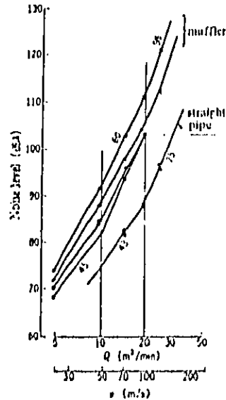
Fig. 7 Flow generated noise level under various mufflers
