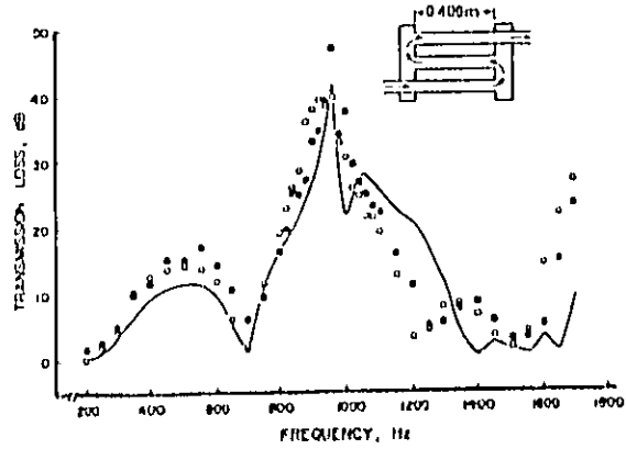
Figure 25. Transmission loss characteristics for combination of S1-CO and C1-SO flow reversing chambers; — is predicted; o is measured without flow and e is measured with a flow speed of 32 m/s
