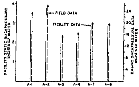
FIGURE 8 Comparison of Field and Facility Muffler Backpressure Ratings
