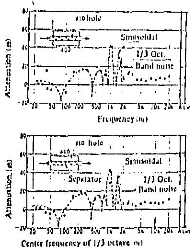
Fig. 1 Effect of test signals to attenuation character characteristic of mufflers
