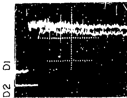
THE EFFECT OF PERFORATED AREA RATIO ON REFLECTED AND TRANSMITTED WAVES. (MACH NO. = 1.13)
