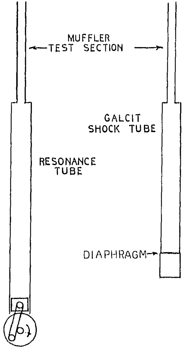
FIGURE 1 THE GEOMETRY OF EXPERIMENTAL FACILITIES
