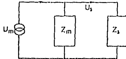
Figure 12 Acoustic model of engine and exhaust system
