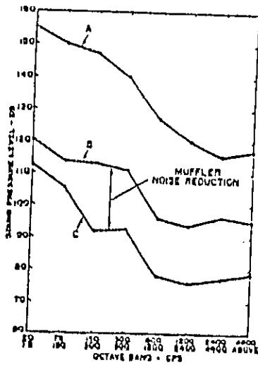
FIGURE 3 Octave Band Analysis of Facility Noise Characteristics
