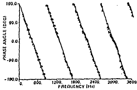
Figure 7. Power Reflection Coefficient and Phase Angle for Open End Tube. Solid Line: Theory; Open Square, Open Triangle: experiment.
