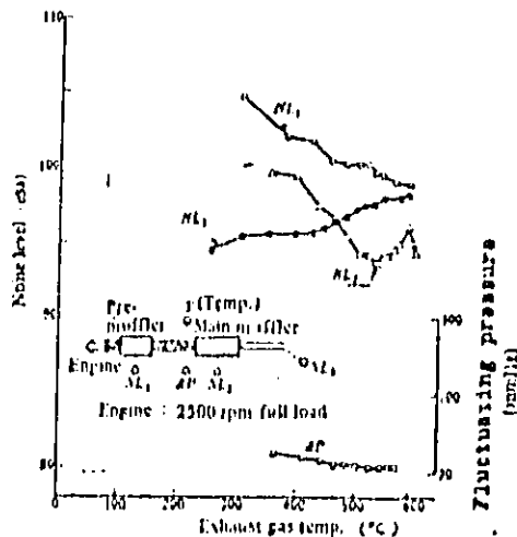
FIG-23 Influence of exhaust gas temperature on exhaust system noise
