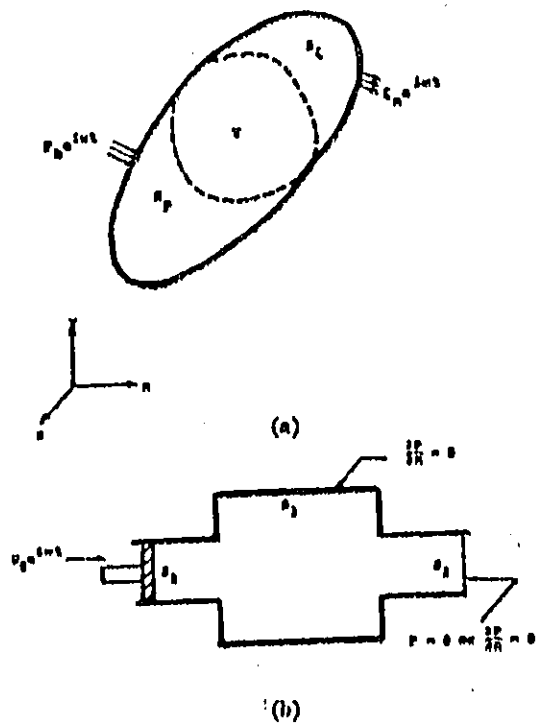
(a) GENERALIZED ACOUSTICAL SYSTEM (b) FORMULATION APPLIED TO EXPANSION CHAMBER MUFFLER
