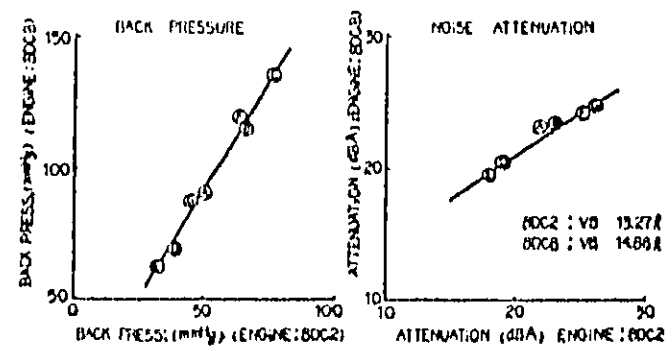
FIG-29 INFLUENCE OF MUFFLER CHARACTERISTICS TO DIFFERENT ENGINE ON A ENGINE BENCH TEST
