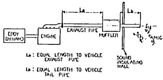
FIG-28 DIAGRAM OF EXHAUST NOISE TEST ON A ENGINE BENCH
