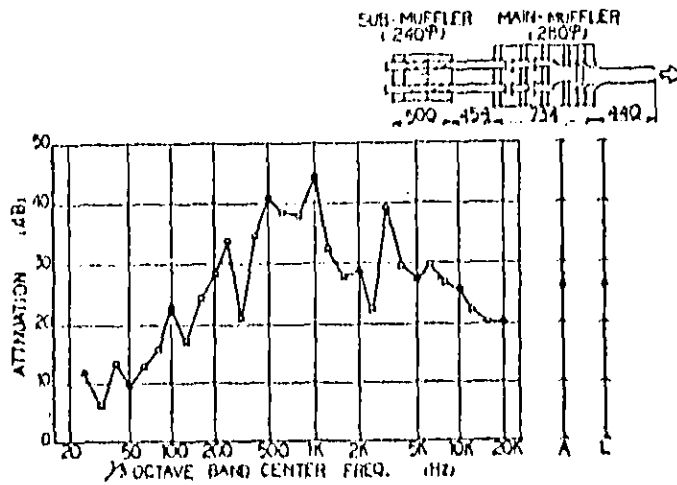
FIG-10 EXAMPLE OF ACOUSTIC ATTENUATION OF MUFFLER
