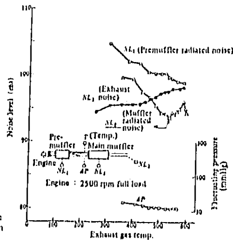
Fig. 20 Influence of exhaust gas temperature on exhaust system noise
