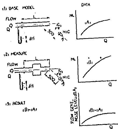
FIG-17 FLOW GENERATED NOISE
