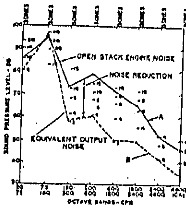
FIGURE 5 Graphic Example of the Effect of Muffling Action upon Exhaust Noise Loudness
