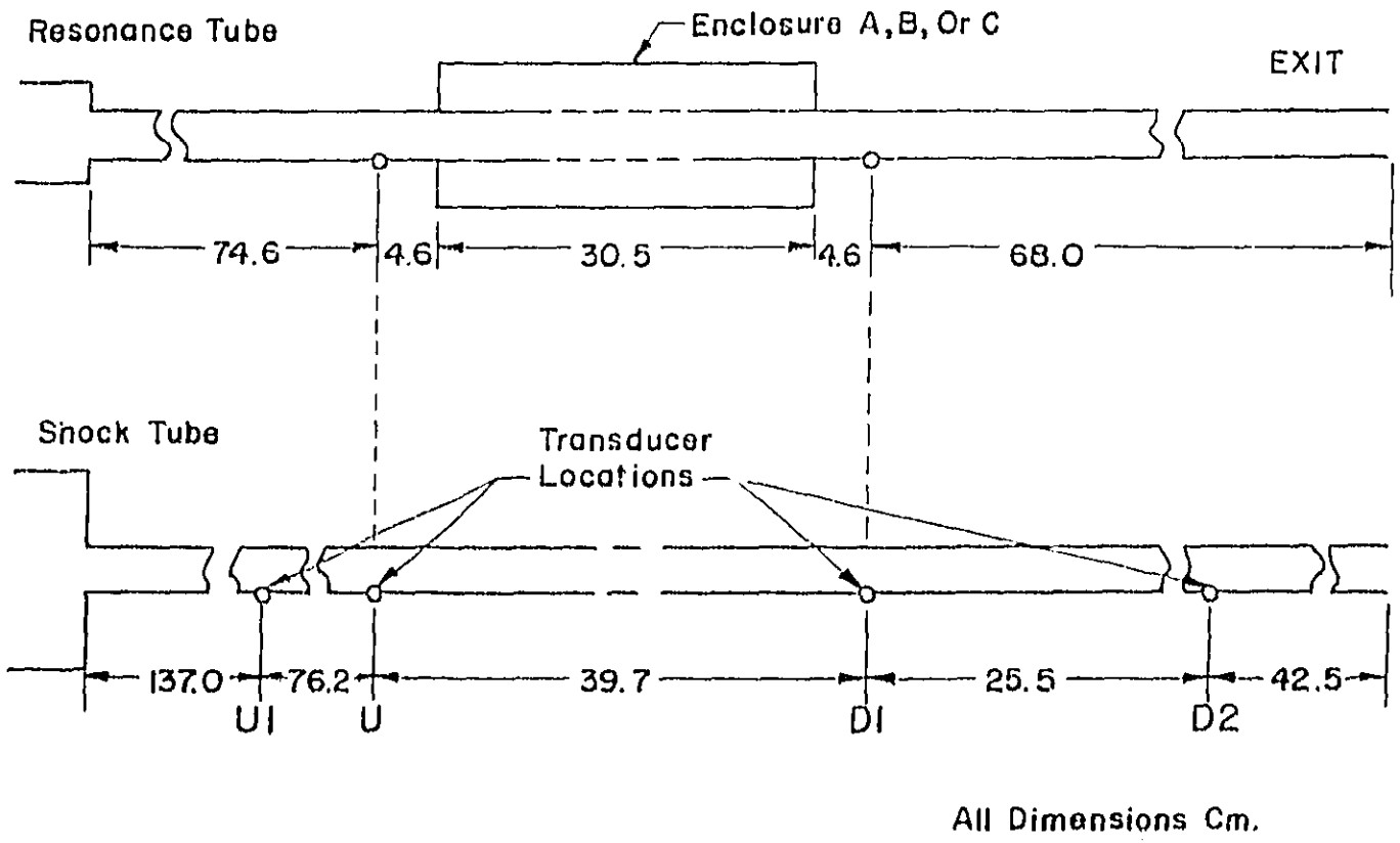
FIGURE 5 PERFORATION SYSTEMS
