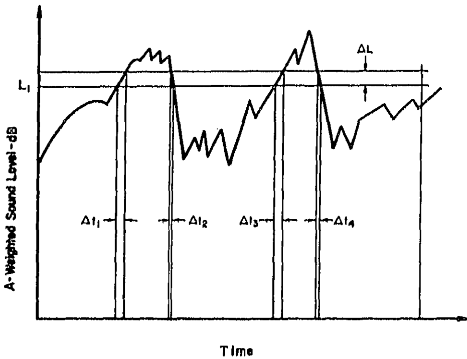
Figure 2-2. Example of the Random Fluctuations of an Urban Noise Signal 5
