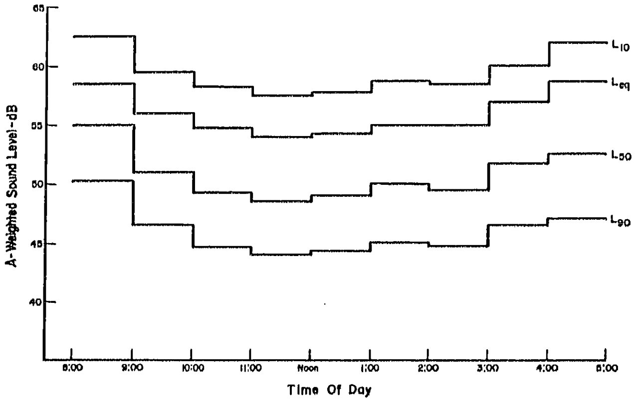
Figure 5-4. Hour-by-Hour County-Wide A-Weighted Sound Levels
