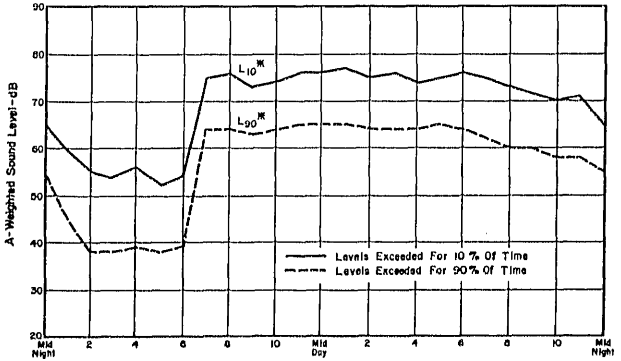
* L 10 and L 90 A-Weighted Sound Levels were determined for each hour of the day. Figure 3-4. Pattern of A-Weighted Sound Levels at Urban Site Over a 24-Hour Period 4
