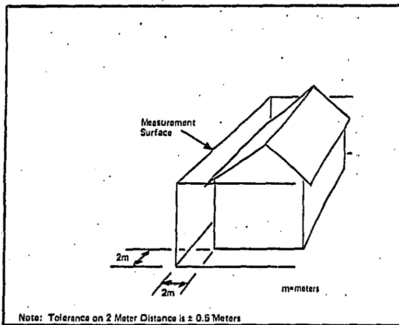
Figure 3. Example of Residential Dwelling Measurement Surface
