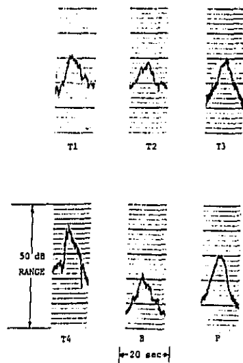
Figure G20. Time histories of the A-weighted sound level for 55 mph passbys of trucks and of a bus. These curves correspond to the 60 m microphones.
