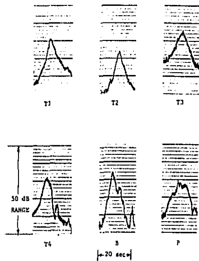
Figure G15. Time histories of the A-weighted sound level for 35 mph passbys of trucks and of a bus. These curves correspond to the 30 m microphone.
