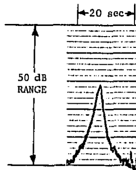
Figure 24. A-weighted sound pressure level time history for a simulated traffic single event passby of automobile No. 7 at 56 km/hr, 15 m microphone.
