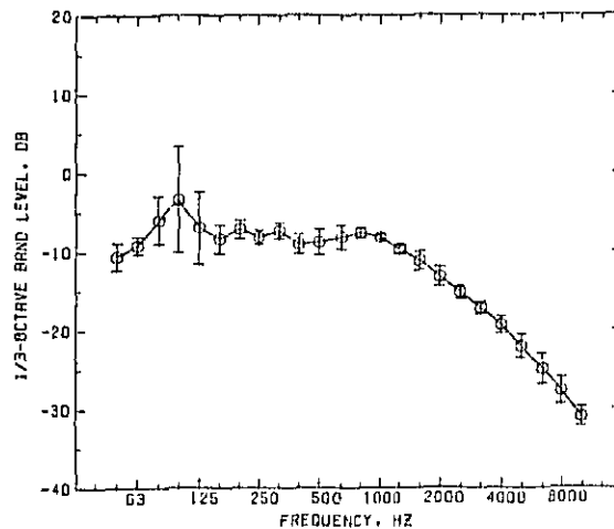
Figure H6. Sound exposure level spectrum relative to the A-weighted sound exposure level, at the 15 m microphone for 55 mph passby of automobiles. The solid circles correspond to the "mean" column in Table H6. The error bars indicate plus and minus one standard deviation about the arithmetic mean.
