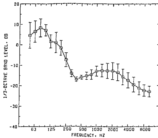
Figure H24. Sound exposure level spectrum relative to the A-weighted sound exposure level, at the 60 m microphone for stop-and-go trucks and a bus. The solid circles correspond to the "mean" column in Table H24. The error bars indicate plus and minus one standard deviation about the arithmetic mean.
