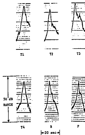
Figure G18. Time histories of the A-weighted sound level for 55 mph passbys of trucks and of a bus. These curves correspond to the 15 m microphones.
