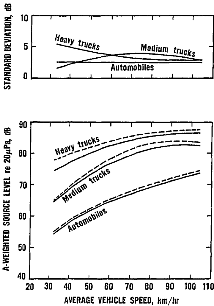
Figure D1. Source levels (lower drawing) and standard deviations of source levels (upper drawing) for automobiles, medium trucks, and heavy trucks [D1].
