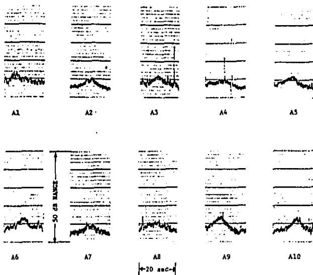
Figure G4. Time histories of the A-weighted sound level for 56 km/hr passbys of automobiles. These curves correspond to the 60 m microphones.
