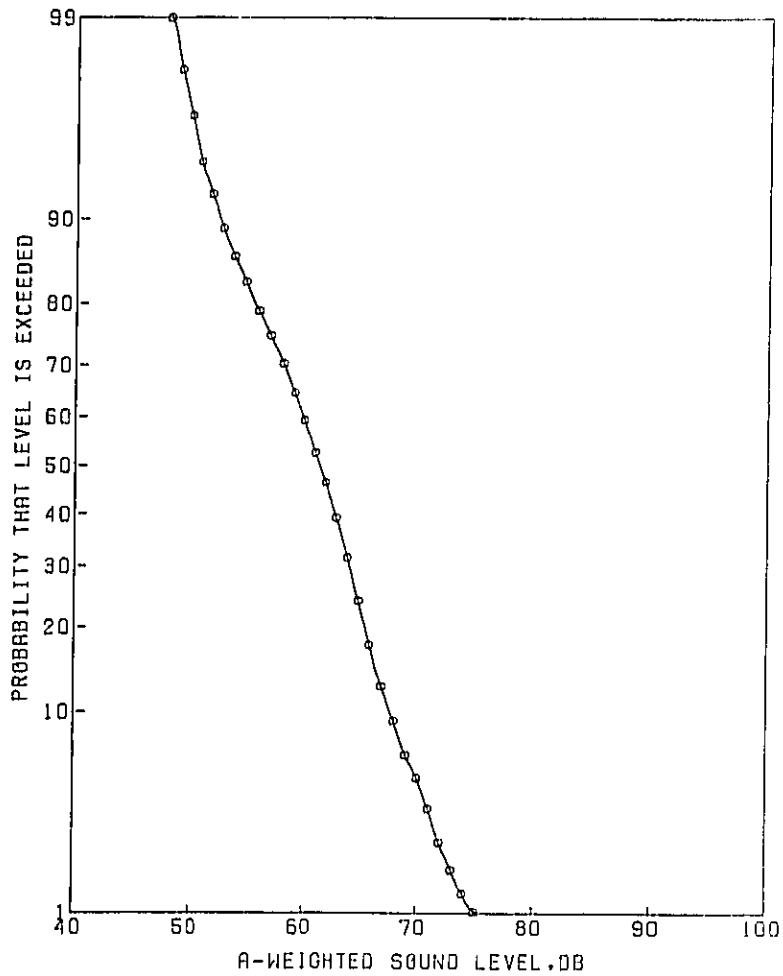
Figure 11. Cumulative probability distribution of A-weighted sound pressure levels for the RT. 28 site, 17 June 1977, 1600 hrs., 15 m microphone.
