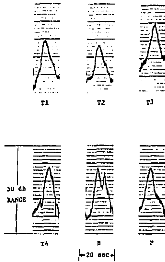
Figure G19. Time histories of the A-weighted sound level for 55 mph passbys of trucks and of a bus. These curves correspond to the 30 m microphones.
