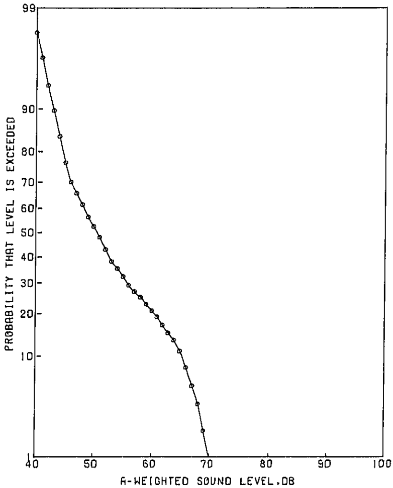
Figure 20. Cumulative probability distribution of A-weighted sound pressure levels for a simulated traffic multiple event of 10 automobiles at 88 km/hr at a flow rate of 300 vehicles per hour, 15 m microphone.
