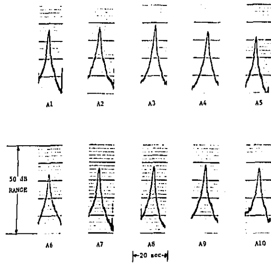
Figure G5. Time histories of the A-weighted sound level for 88 km/hr passbys of automobiles. These curves correspond to the 7.5 m microphone.
