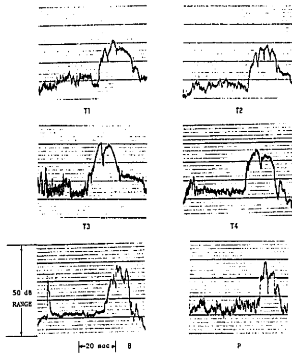
Figure G23. Time histories of the A-weighted sound level for stop-and-go passbys of trucks and of a bus. These curves correspond to the 30 m microphones.
