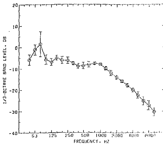
Figure H2. Sound exposure level spectra relative to the A-weighted sound exposure level, at the 15 m microphone for 35 mph passbys of automobiles. The solid circles correspond to the "mean" column in Table H2. The error bars indicate plus and minus one standard deviation about the arithmetic mean.
