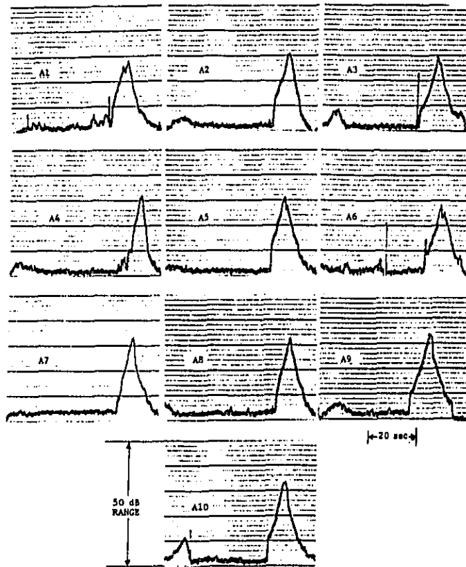
Figure G 9. Time histories of the A-weighted sound level for stop-and-go passbys of automobiles. These curves correspond to the 7.5 m microphones.
