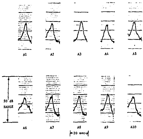
Figure G7. Time histories of the A-weighted sound level for 88 km/hr passbys of automobiles. These curves correspond to the 30 m microphones.
