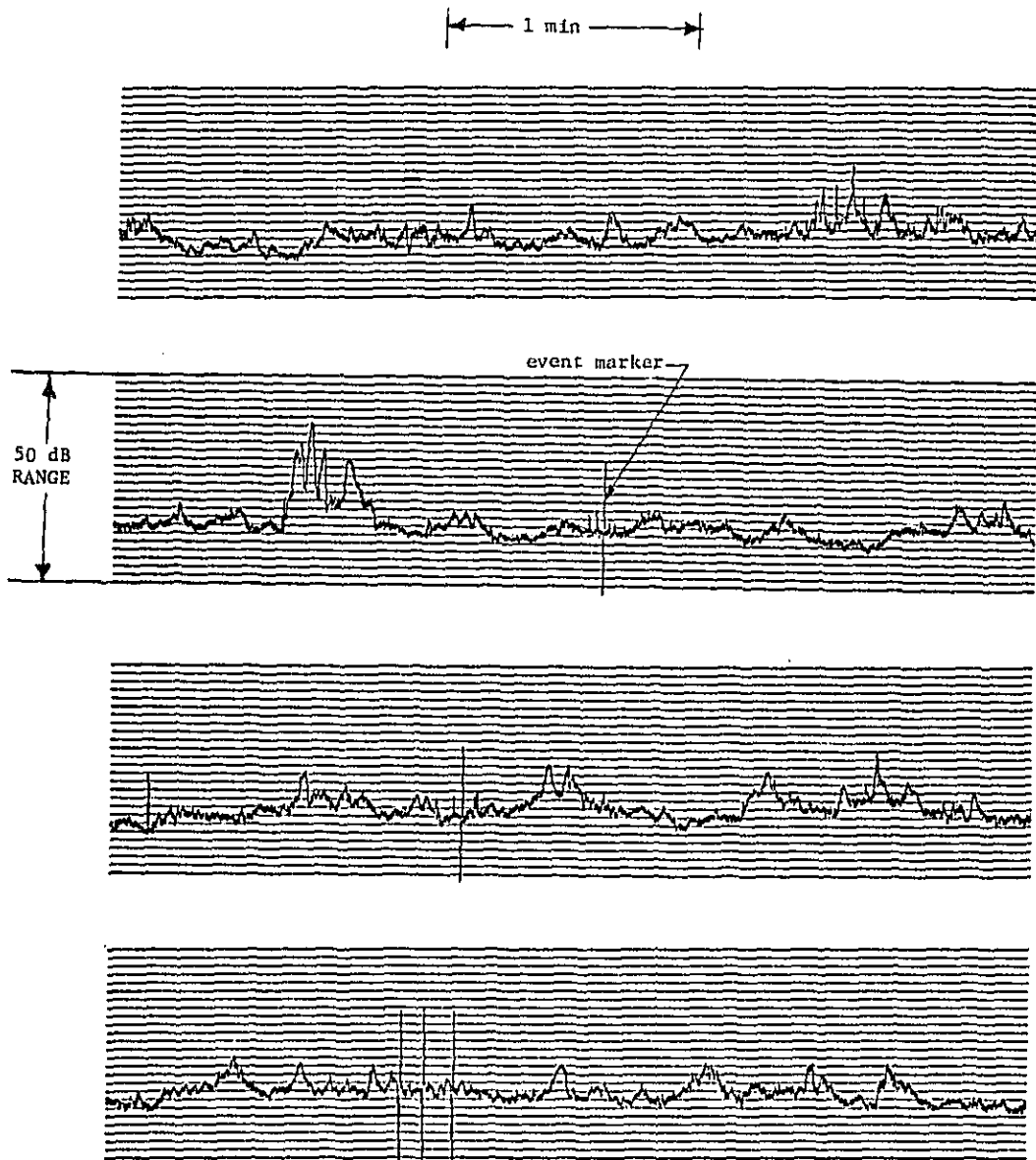
Figure 9. A-weighted sound pressure level time history for the 355 and Q. O. RD. site, 24 June 1977, 1600 hrs., 15 m microphone.
