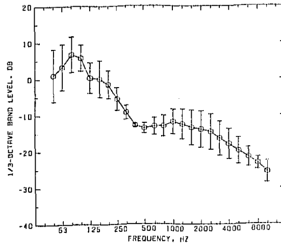
Figure H23. Sound exposure level spectrum relative to the A-weighted sound exposure level, at the 30 m microphones for stop-and-go trucks and a bus. The solid circles correspond to the "mean" column in Table H23. The error bars indicate plus and minus one standard deviation about the arithmetic mean.
