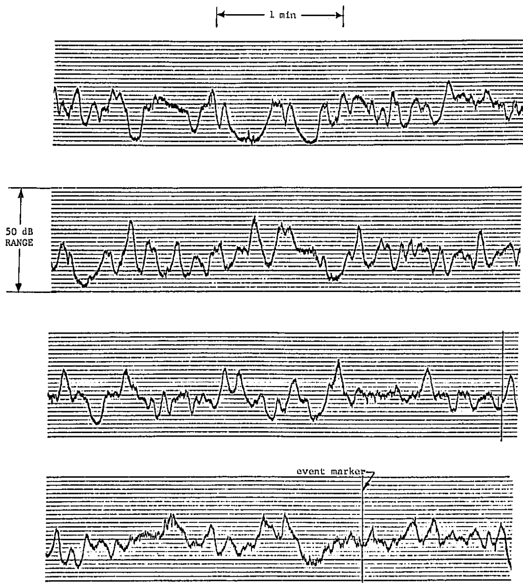
Figure 8. A-weighted sound pressure level time history for the GUDE DR. site, 16 June 1977, 1600 hrs., 15 m microphone.
