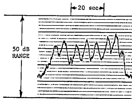
Figure 18. A-weighted sound pressure level time history for a simulated traffic multiple event passby of 7 automobiles with 3 gaps (after peaks 2, 3, and 5) at a speed of 56 km/hr and flow rate of 660 vehicles per hour, 15 m microphone.
