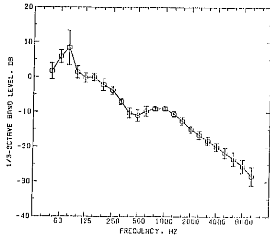
Figure III. Sound exposure level spectrum relative to the A-weighted sound exposure level, at the 30 m microphone for 35 mph passbys of automobiles. The solid circles correspond to the "mean" column in Table III. The error bars indicate plus and minus one standard deviation about the arithmetic mean.
