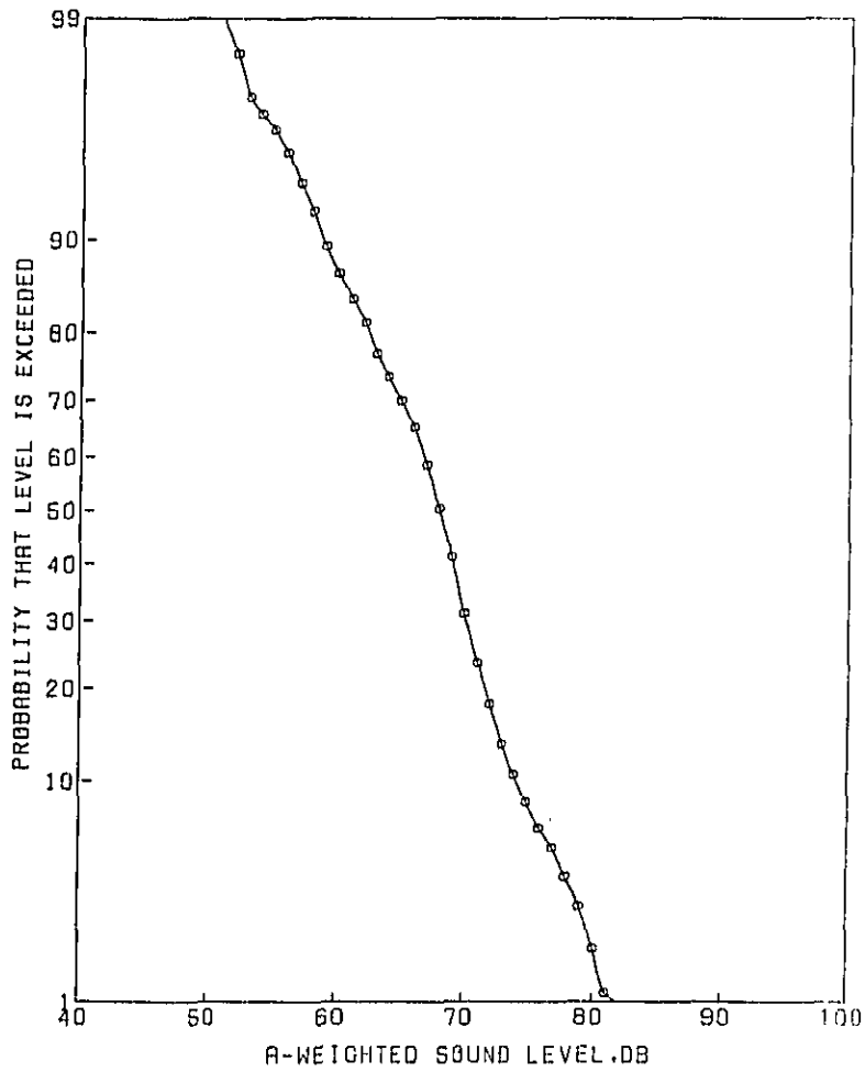
Figure 12. Cumulative probability distribution of A-weighted sound pressure levels for the GUDE DR. site, 16 June 1977, 1600 hrs., 15 m microphone.
