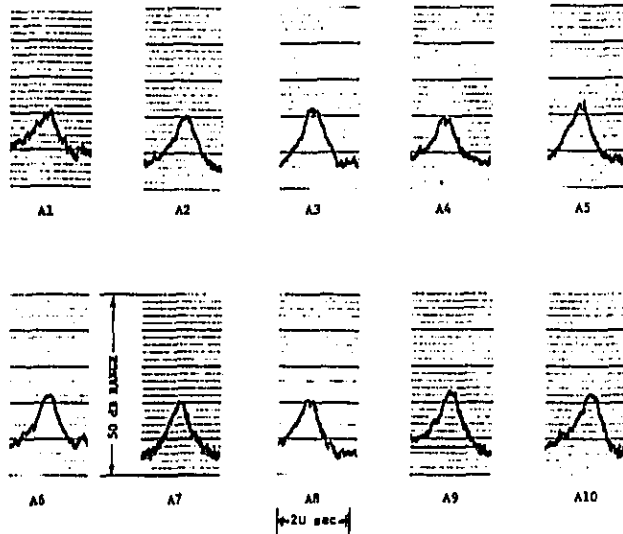
Figure G3. Time histories of the A-weighted sound level for 56 km/hr passbys of automobiles. These curves correspond to the 30 m microphones.
