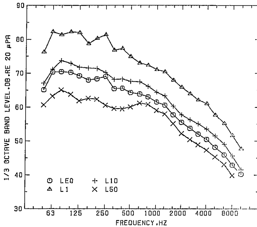
Figure 4. 1/3-octave band LEQ, L1, L10, and L50 spectra for the GUDE DR. site, 16 June 1977, 1600, hrs., 15 m microphone, recording duration of 14.5 min.
