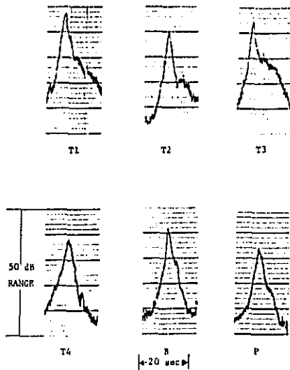
Figure G14. Time histories of the A-weighted sound level for 35 mph passbys of trucks and of a bus. These curves correspond to the 13 m microphones.
