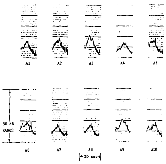
Figure G8. Time histories of the A-weighted sound level for 88 km/hr passbys of automobiles. These curves correspond to the 60 m microphones.
