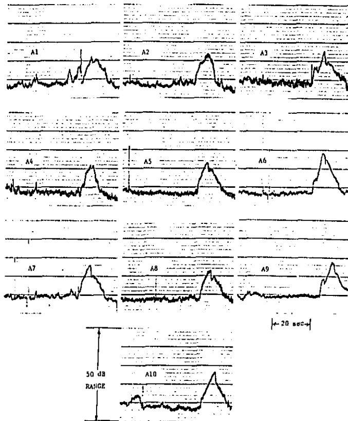
Figure G11. Time histories of the A-weighted sound level for stop-and-go passby of automobiles. These curves correspond to the 30 is microphone.
