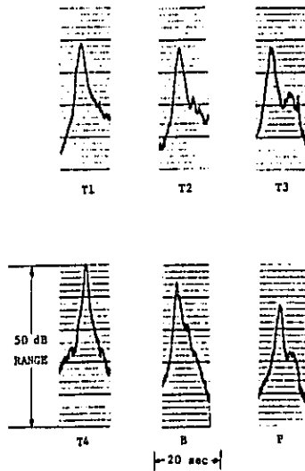
Figure G17. Time histories of the A-weighted sound level for 55 mph passbys of trucks and of a bus. These curves correspond to the 7.5 m microphones.
