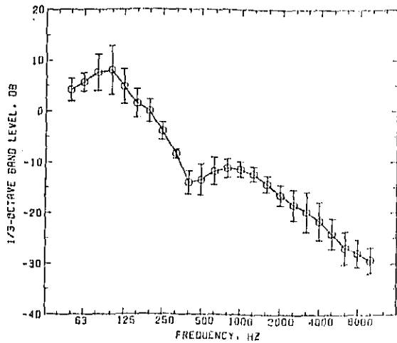
Figure H8. Sound exposure level spectrum relative to the A-weighted sound exposure level, at the 60 m microphone for 55 mph passbys of automobiles. The solid circles correspond to the "mean" column in Table H8. The error bars indicate plus and minus one standard deviation about the arithmetic mean.
