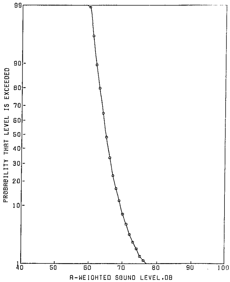
Figure 13. Cumulative probability distribution of A-weighted sound pressure levels for the 355 and Q.O. RD. site, 24 June 1977, 1600 hrs., 15 m microphone.
