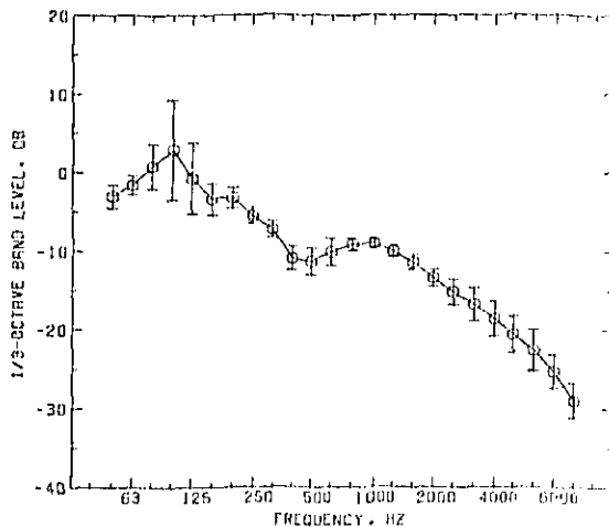
Figure H7. Sound exposure level spectrum relative to the A-weighted sound exposure level, at the 30 m microphone for 55 mph passbys of automobiles. The solid circles correspond to the "mean" column in Table H7. The error bars indicate plus and minus one standard deviation about the arithmetic mean.
