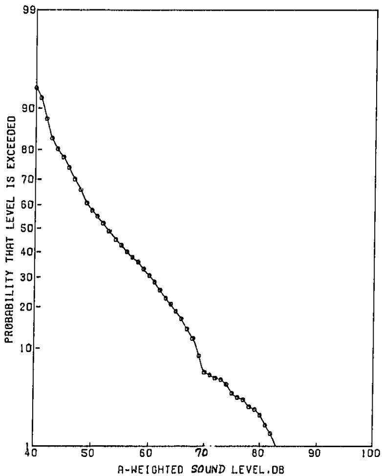
Figure I2. Cumulative probability distribution of A-weighted sound pressure levels for the time history obtained by (computer) dubbing of the single-event recording S-55-T3 twice into the multiple-event recording M-55A-8B.
