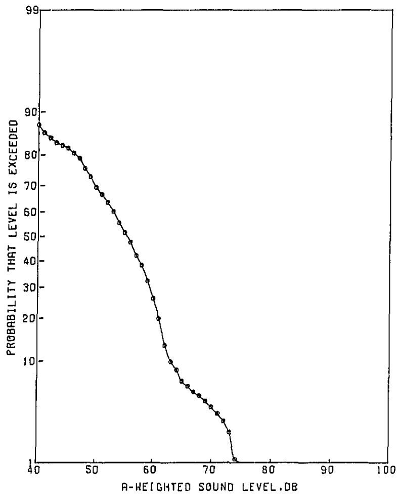
Figure 11. Cumulative probability distribution of A-weighted sound pressure levels for the synthesized time history obtained by (computer) dubbing of single-event recording S-35-T2 into the multiple-event recording M-35B-9.
