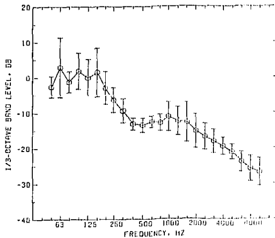
Figure H15. Sound exposure level spectrum relative to the A-weighted sound exposure level, at the 30 m microphone for 35 mph passbys of trucks and of a bus. The solid circles correspond to the "mean" column in Table H15. The error bars indicate plus and minus one standard deviation about the arithmetic mean.
