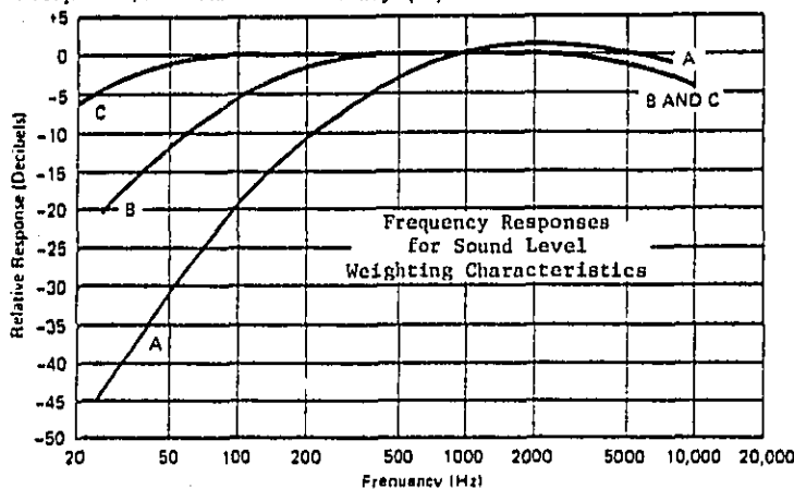
Figure 7-1. Frequency responses for sound level weighting characteristics.
