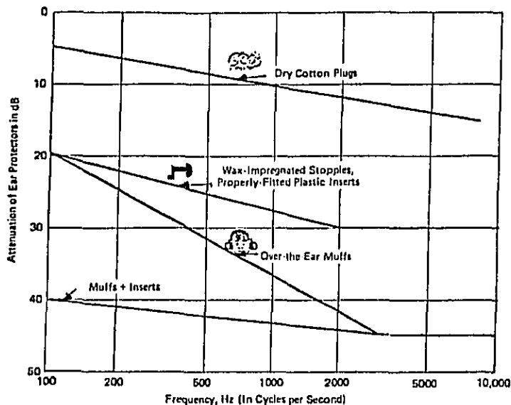
Figure 2-10. Sound attenuation characteristics of various types of ear protectors Source: Ref. 23
