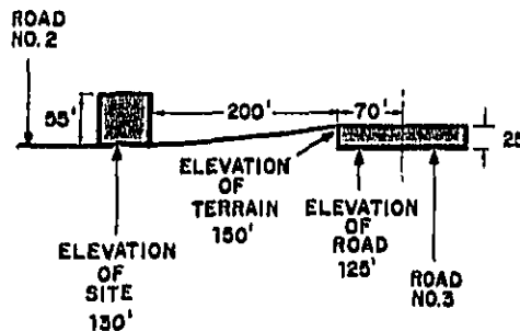
Detail of Site Showing the Measurements Necessary for a Barrier Adjustment.
