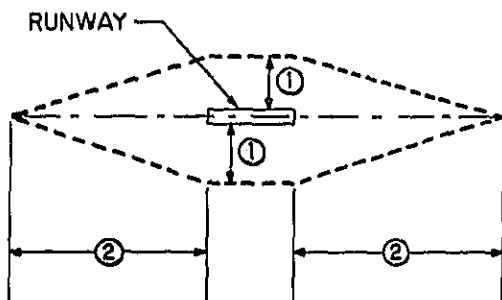
Construction of Approximate NEF Contours Using the Distances in Table II.
