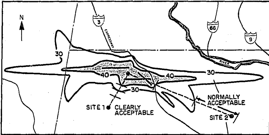
Example of NEF Contours
