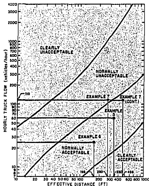
Example of How Figure 3 is Used to Evaluate the Site's Exposure to Truck Noise.
