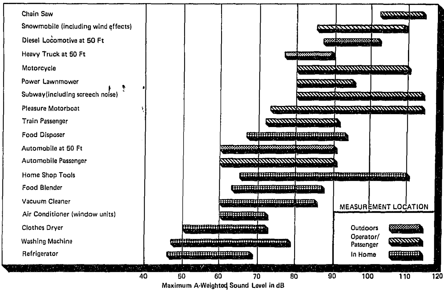
FIGURE 1. TYPICAL RANGE OF COMMON SOUNDS
