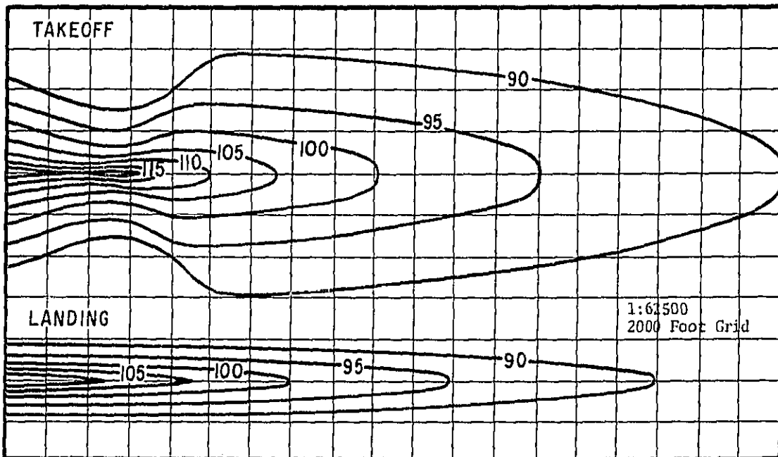
(a) Two-Engine Turbopfan Aircraft
