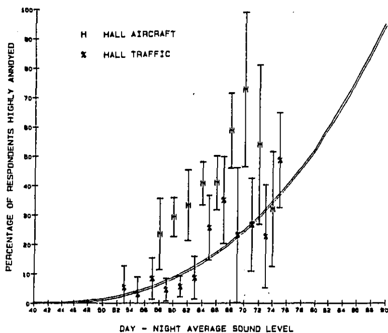
FIG. 2. Relationship of data from Aircraft-Traffic comparison to 1978 synthesis curve.
